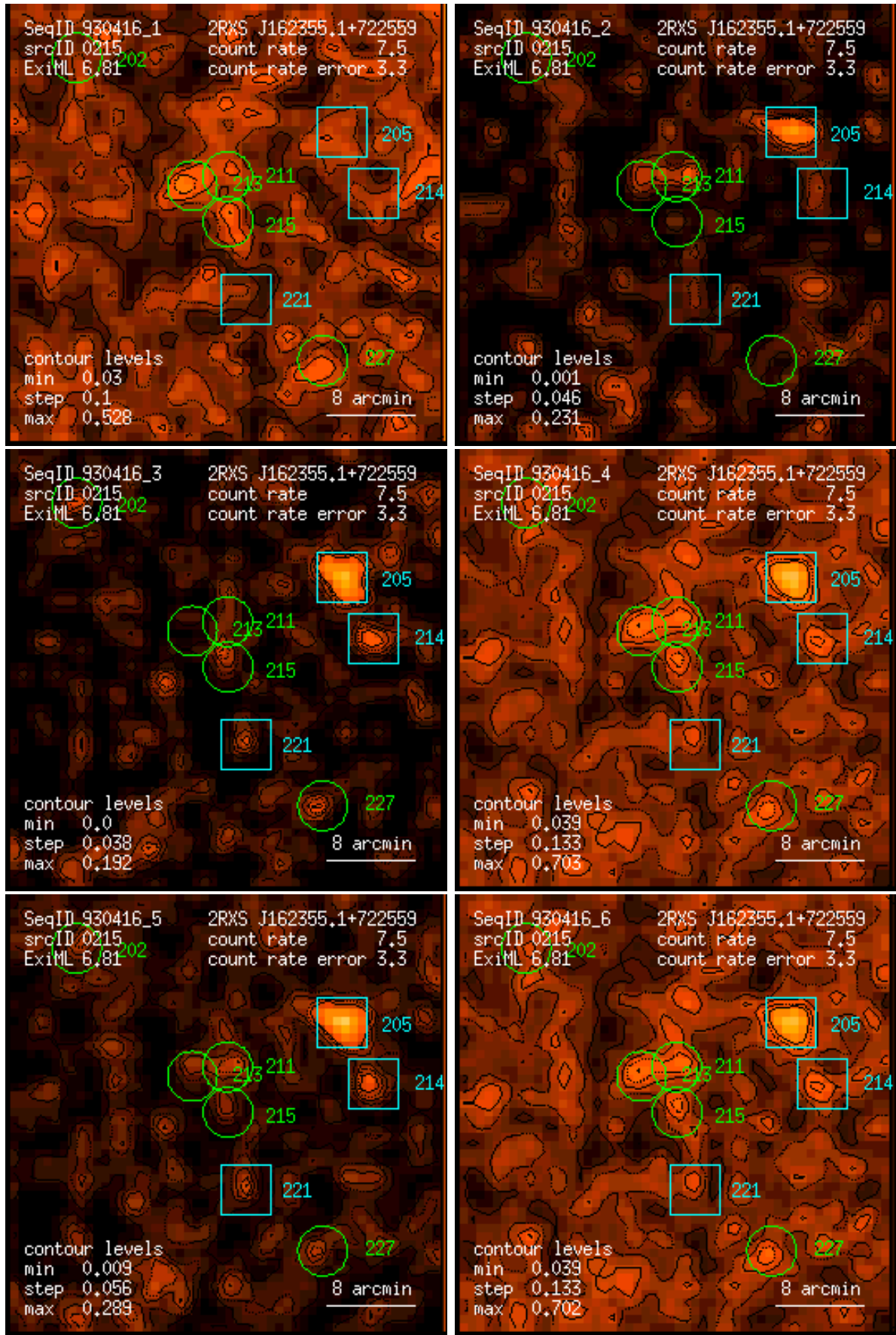
Figure 215: RASS 930416: detection 0215: band rate images, Gaussian filter: (1) PSPC channels 11 – 41, (2) 52 – 90, (3) 91 – 201, (4) 11 – 235, (5) 52 – 201, (6) 11 – 201. Broad band rates in counts/ks. Band rate contour levels in counts/ks/arcmin 2 .
