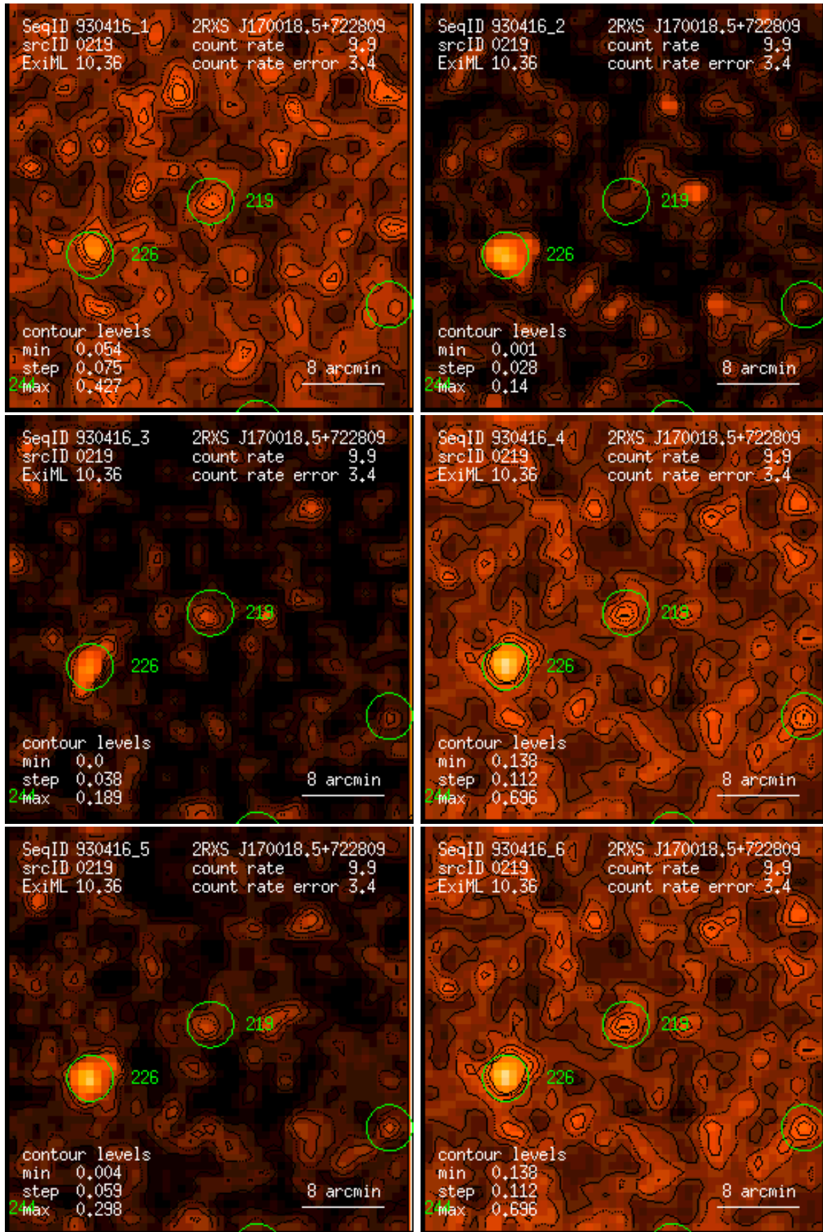
Figure 219: RASS 930416: detection 0219: band rate images, Gaussian filter: (1) PSPC channels 11 – 41, (2) 52 – 90, (3) 91 – 201, (4) 11 – 235, (5) 52 – 201, (6) 11 – 201. Broad band rates in counts/ks. Band rate contour levels in counts/ks/arcmin 2 .
