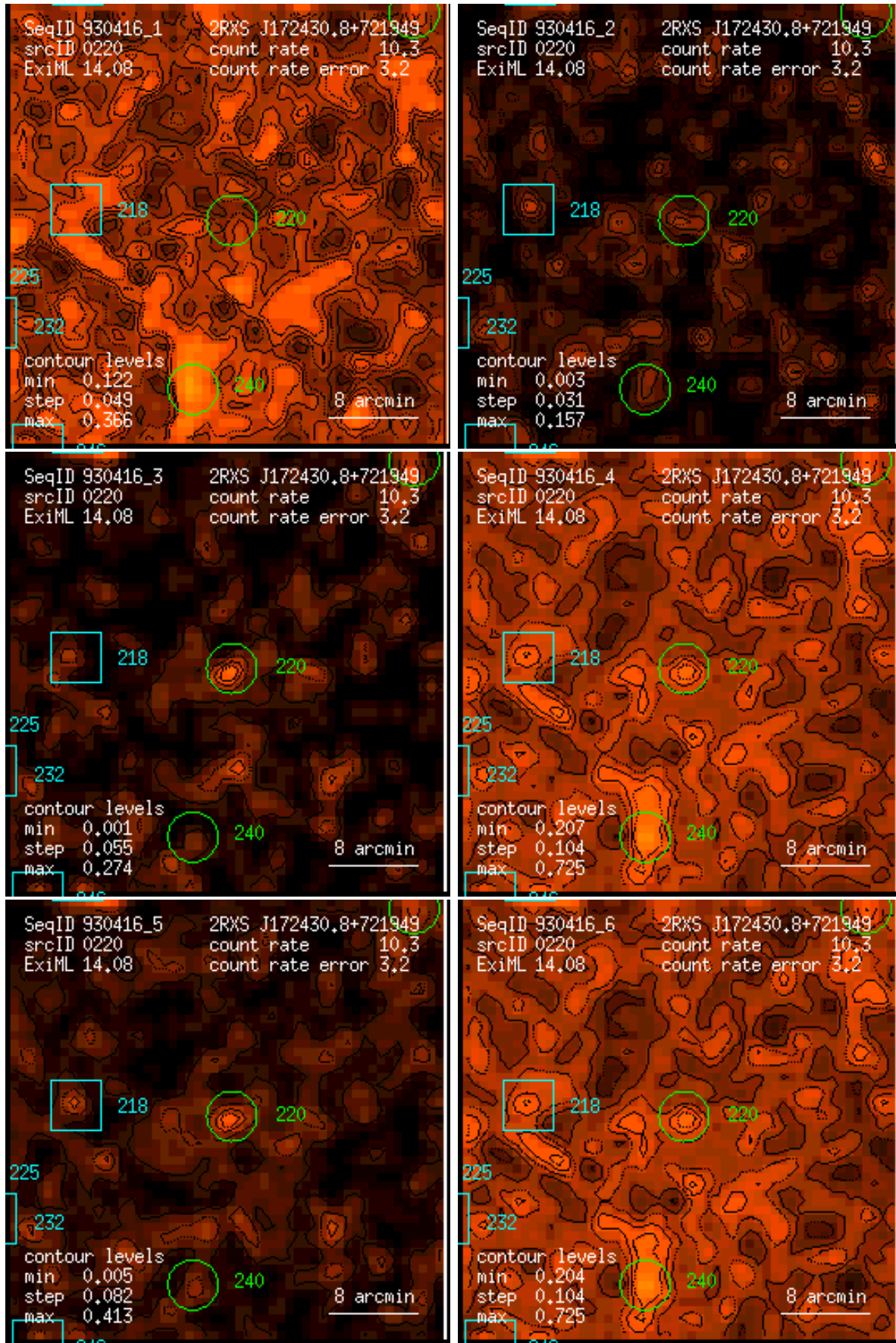
Figure 220: RASS 930416: detection 0220: band rate images, Gaussian filter: (1) PSPC channels 11 – 41, (2) 52 – 90, (3) 91 – 201, (4) 11 – 235, (5) 52 – 201, (6) 11 – 201. Broad band rates in counts/ks. Band rate contour levels in counts/ks/arcmin 2 .
