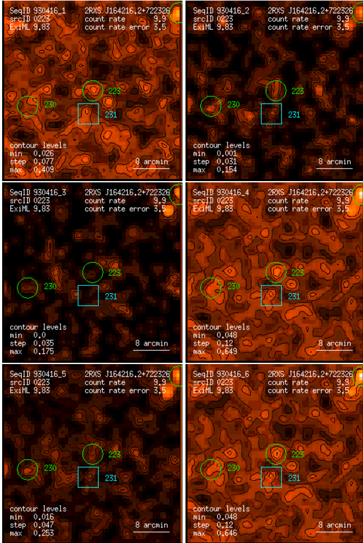
Figure 223: RASS 930416: detection 0223: band rate images, Gaussian filter: (1) PSPC channels 11 – 41, (2) 52 – 90, (3) 91 – 201, (4) 11 – 235, (5) 52 – 201, (6) 11 – 201. Broad band rates in counts/ks. Band rate contour levels in counts/ks/arcmin 2 .
