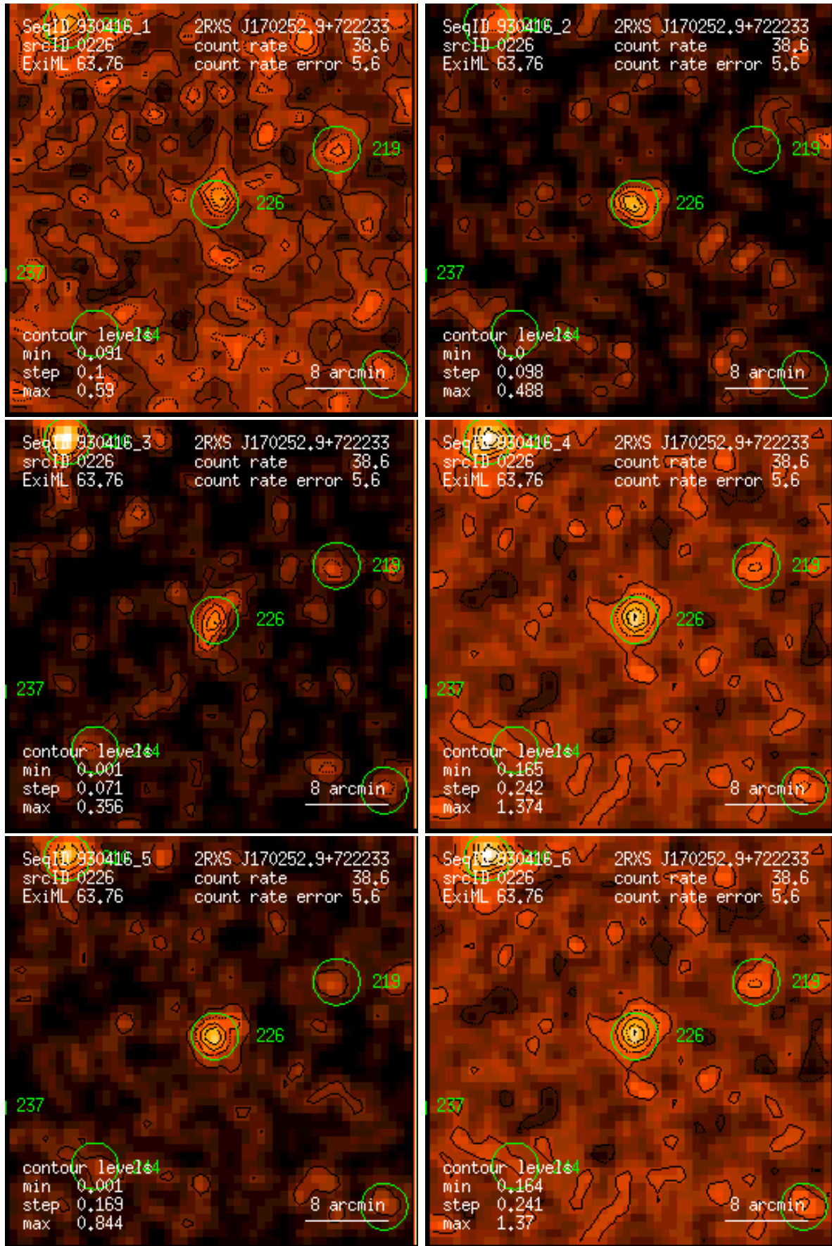
Figure 226: RASS 930416: detection 0226: band rate images, Gaussian filter: (1) PSPC channels 11 – 41, (2) 52 – 90, (3) 91 – 201, (4) 11 – 235, (5) 52 – 201, (6) 11 – 201. Broad band rates in counts/ks. Band rate contour levels in counts/ks/arcmin 2 .
