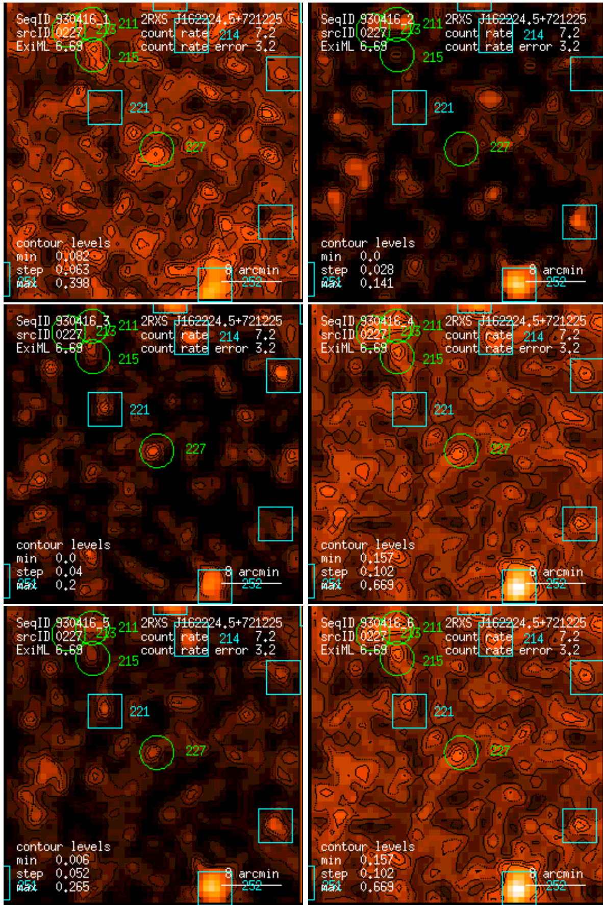
Figure 227: RASS 930416: detection 0227: band rate images, Gaussian filter: (1) PSPC channels 11 – 41, (2) 52 – 90, (3) 91 – 201, (4) 11 – 235, (5) 52 – 201, (6) 11 – 201. Broad band rates in counts/ks. Band rate contour levels in counts/ks/arcmin 2 .
