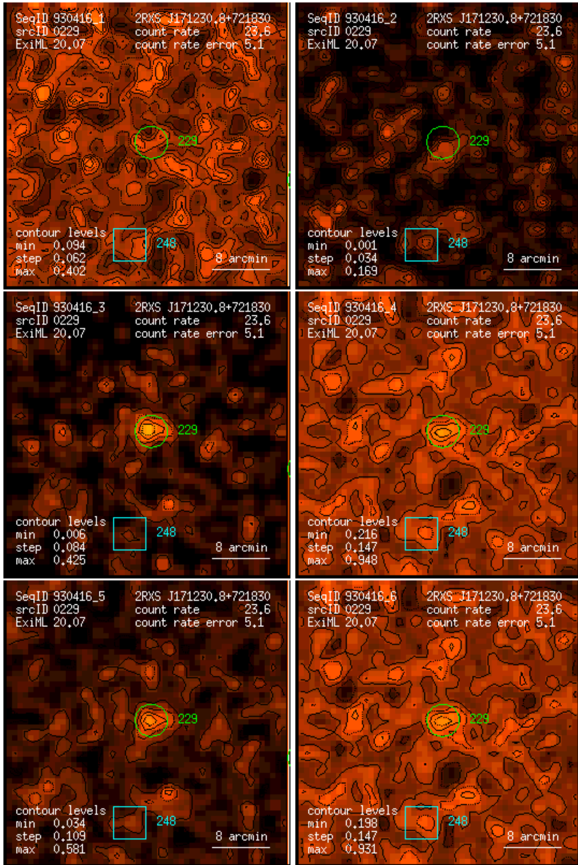
Figure 229: RASS 930416: detection 0229: band rate images, Gaussian filter: (1) PSPC channels 11 – 41, (2) 52 – 90, (3) 91 – 201, (4) 11 – 235, (5) 52 – 201, (6) 11 – 201. Broad band rates in counts/ks. Band rate contour levels in counts/ks/arcmin 2 .
