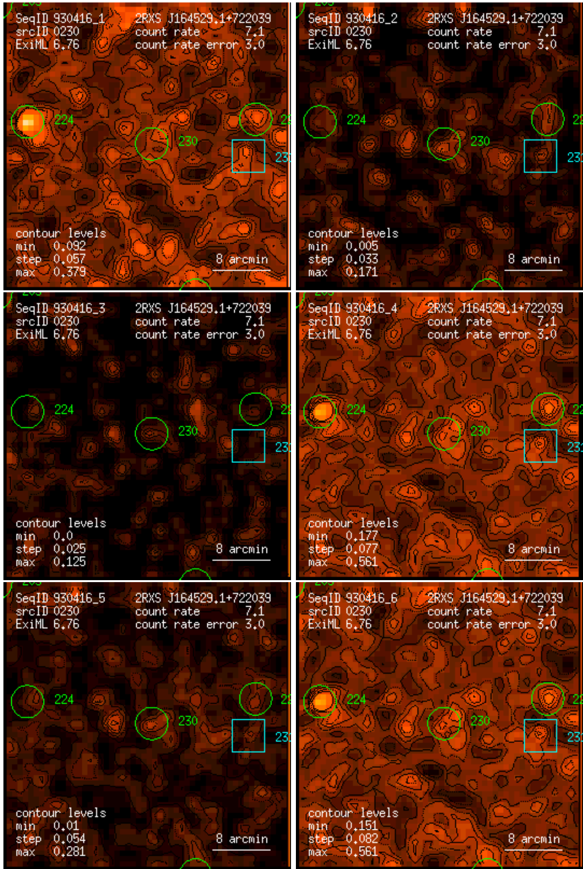
Figure 230: RASS 930416: detection 0230: band rate images, Gaussian filter: (1) PSPC channels 11 – 41, (2) 52 – 90, (3) 91 – 201, (4) 11 – 235, (5) 52 – 201, (6) 11 – 201. Broad band rates in counts/ks. Band rate contour levels in counts/ks/arcmin 2 .
