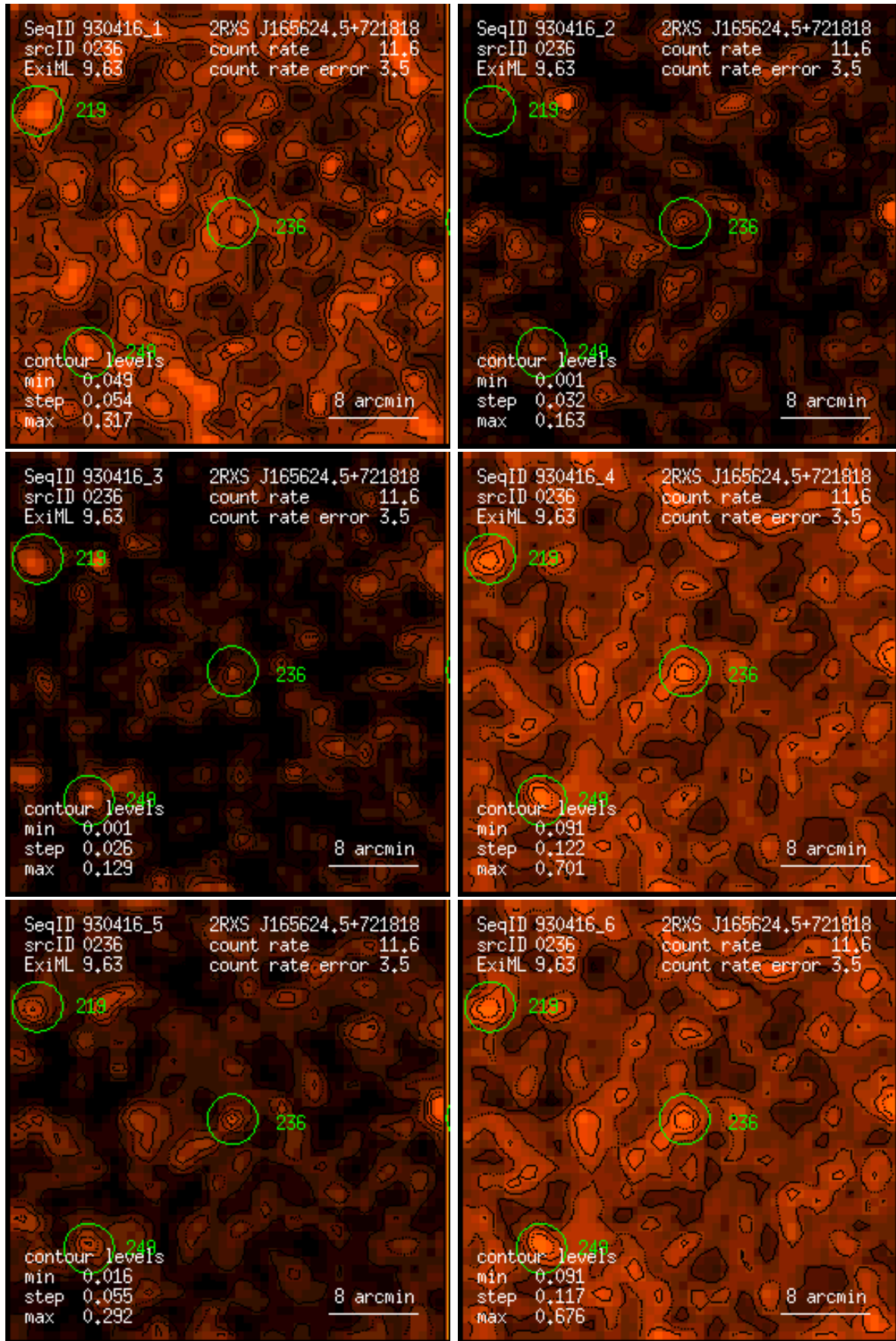
Figure 236: RASS 930416: detection 0236: band rate images, Gaussian filter: (1) PSPC channels 11 – 41, (2) 52 – 90, (3) 91 – 201, (4) 11 – 235, (5) 52 – 201, (6) 11 – 201. Broad band rates in counts/ks. Band rate contour levels in counts/ks/arcmin 2 .
