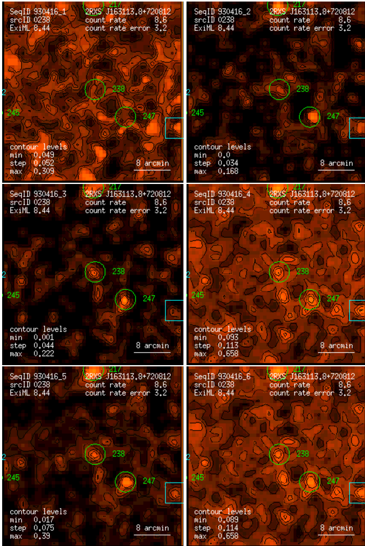
Figure 238: RASS 930416: detection 0238: band rate images, Gaussian filter: (1) PSPC channels 11 – 41, (2) 52 – 90, (3) 91 – 201, (4) 11 – 235, (5) 52 – 201, (6) 11 – 201. Broad band rates in counts/ks. Band rate contour levels in counts/ks/arcmin 2 .
