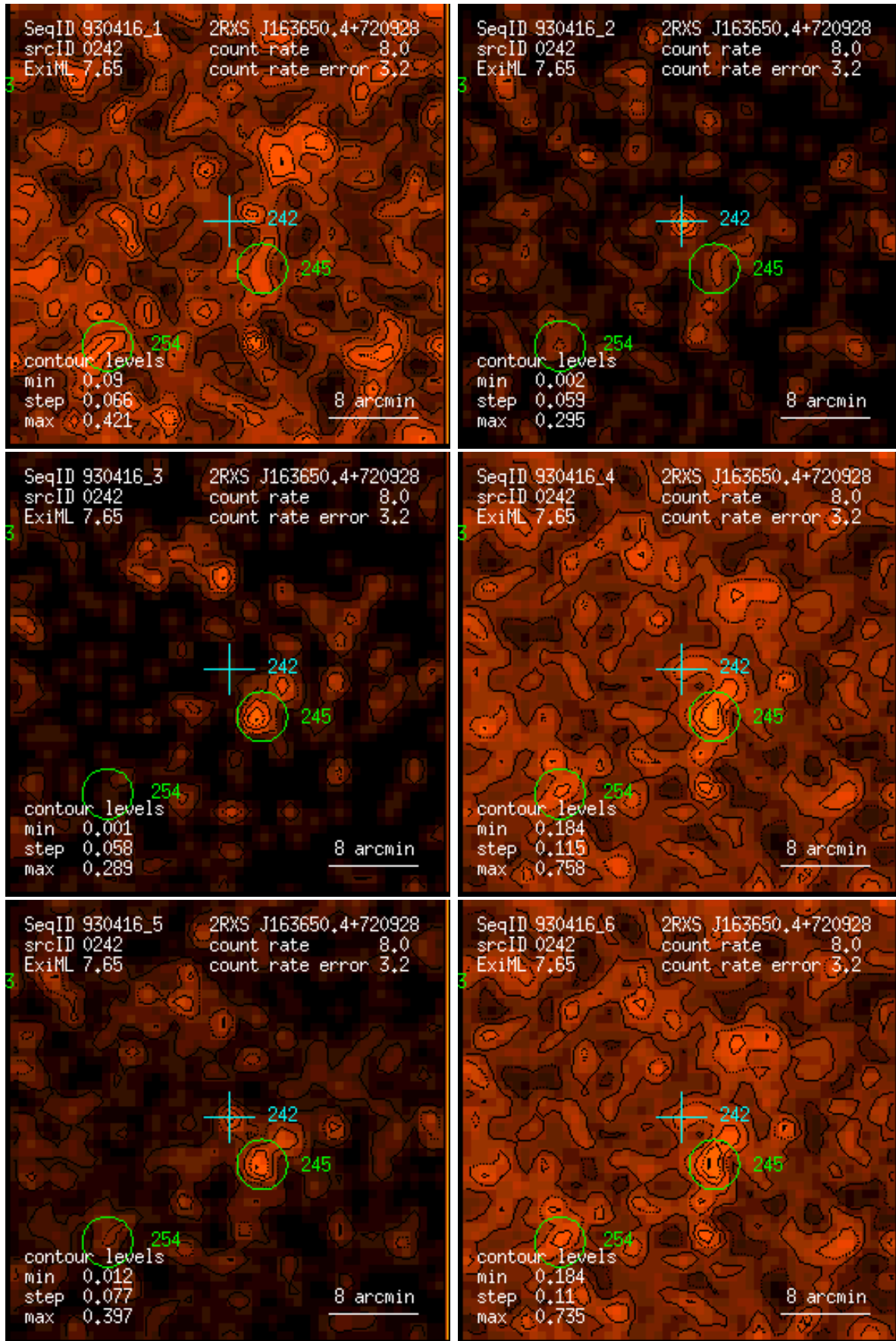
Figure 242: RASS 930416: detection 0242: band rate images, Gaussian filter: (1) PSPC channels 11 – 41, (2) 52 – 90, (3) 91 – 201, (4) 11 – 235, (5) 52 – 201, (6) 11 – 201. Broad band rates in counts/ks. Band rate contour levels in counts/ks/arcmin 2 .
