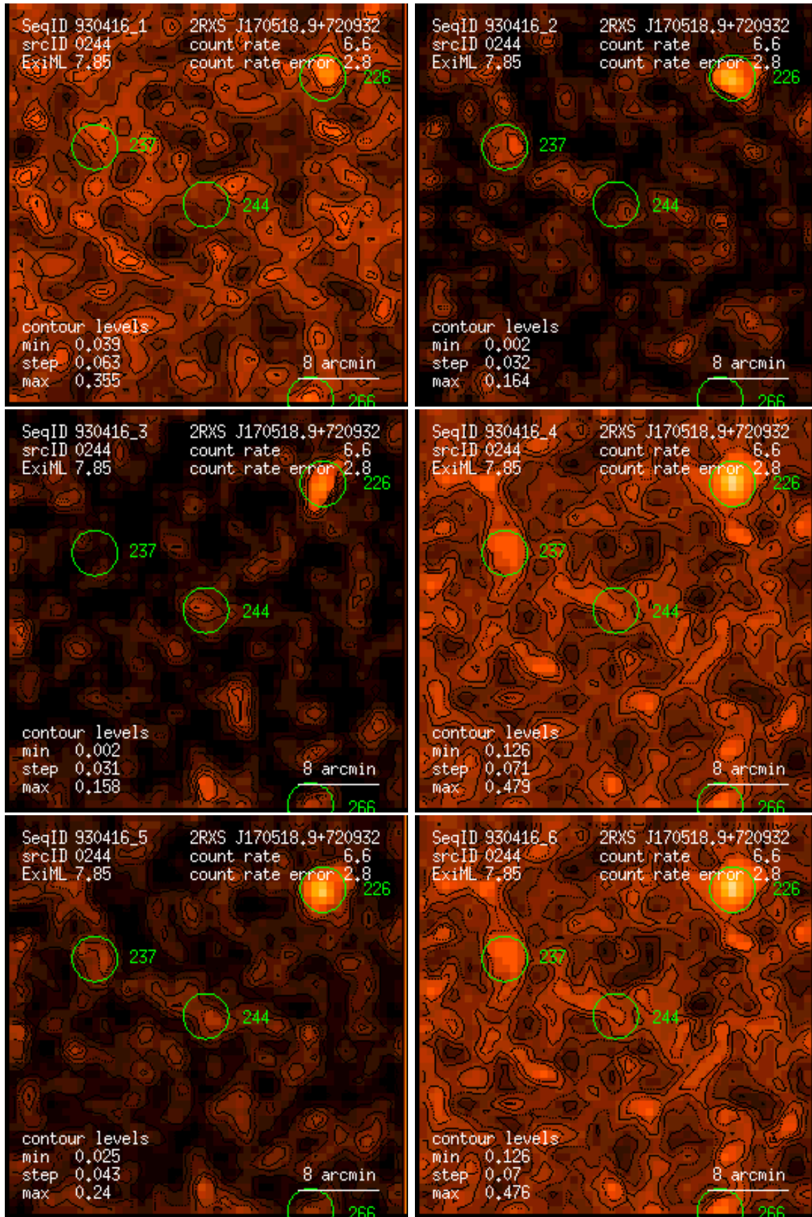
Figure 244: RASS 930416: detection 0244: band rate images, Gaussian filter: (1) PSPC channels 11 – 41, (2) 52 – 90, (3) 91 – 201, (4) 11 – 235, (5) 52 – 201, (6) 11 – 201. Broad band rates in counts/ks. Band rate contour levels in counts/ks/arcmin 2 .
