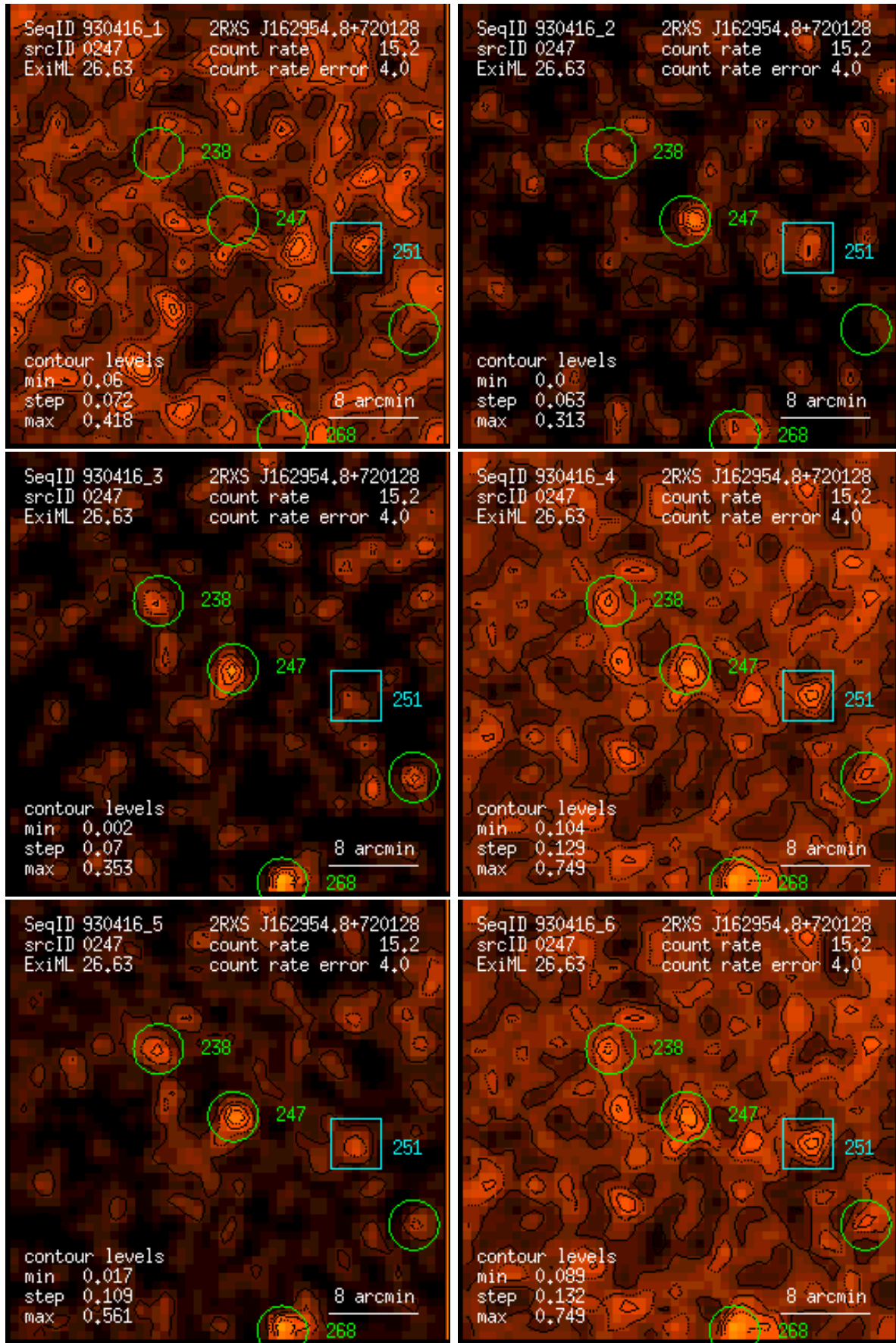
Figure 247: RASS 930416: detection 0247: band rate images, Gaussian filter: (1) PSPC channels 11 – 41, (2) 52 – 90, (3) 91 – 201, (4) 11 – 235, (5) 52 – 201, (6) 11 – 201. Broad band rates in counts/ks. Band rate contour levels in counts/ks/arcmin 2 .
