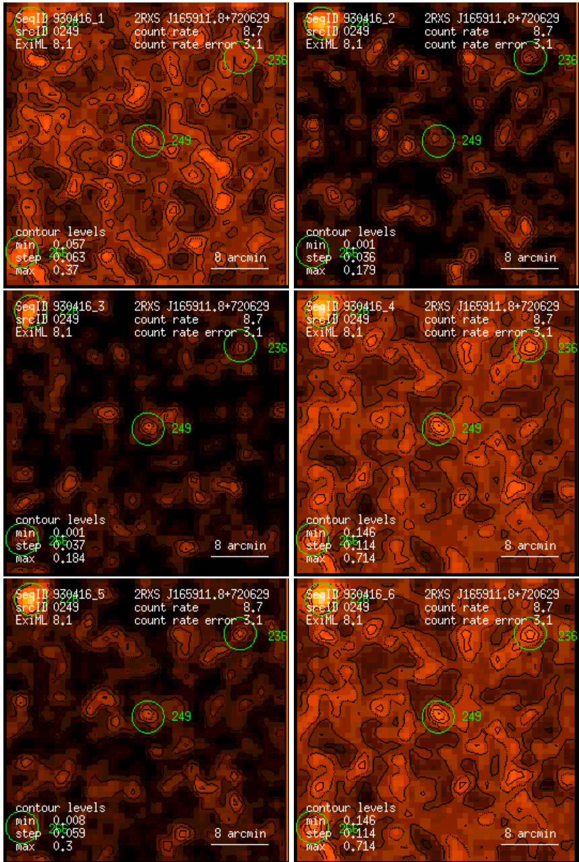
Figure 249: RASS 930416: detection 0249: band rate images, Gaussian filter: (1) PSPC channels 11 – 41, (2) 52 – 90, (3) 91 – 201, (4) 11 – 235, (5) 52 – 201, (6) 11 – 201. Broad band rates in counts/ks. Band rate contour levels in counts/ks/arcmin 2 .
