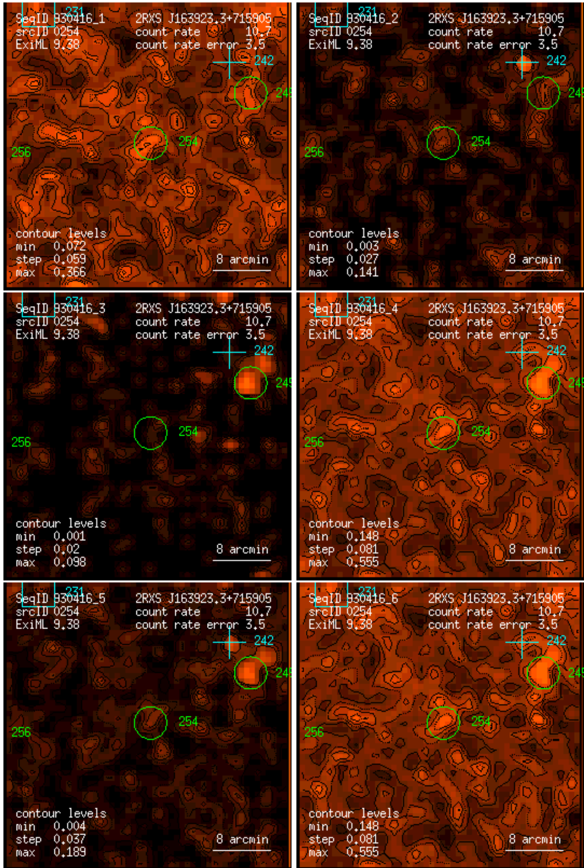
Figure 254: RASS 930416: detection 0254: band rate images, Gaussian filter: (1) PSPC channels 11 – 41, (2) 52 – 90, (3) 91 – 201, (4) 11 – 235, (5) 52 – 201, (6) 11 – 201. Broad band rates in counts/ks. Band rate contour levels in counts/ks/arcmin 2 .
