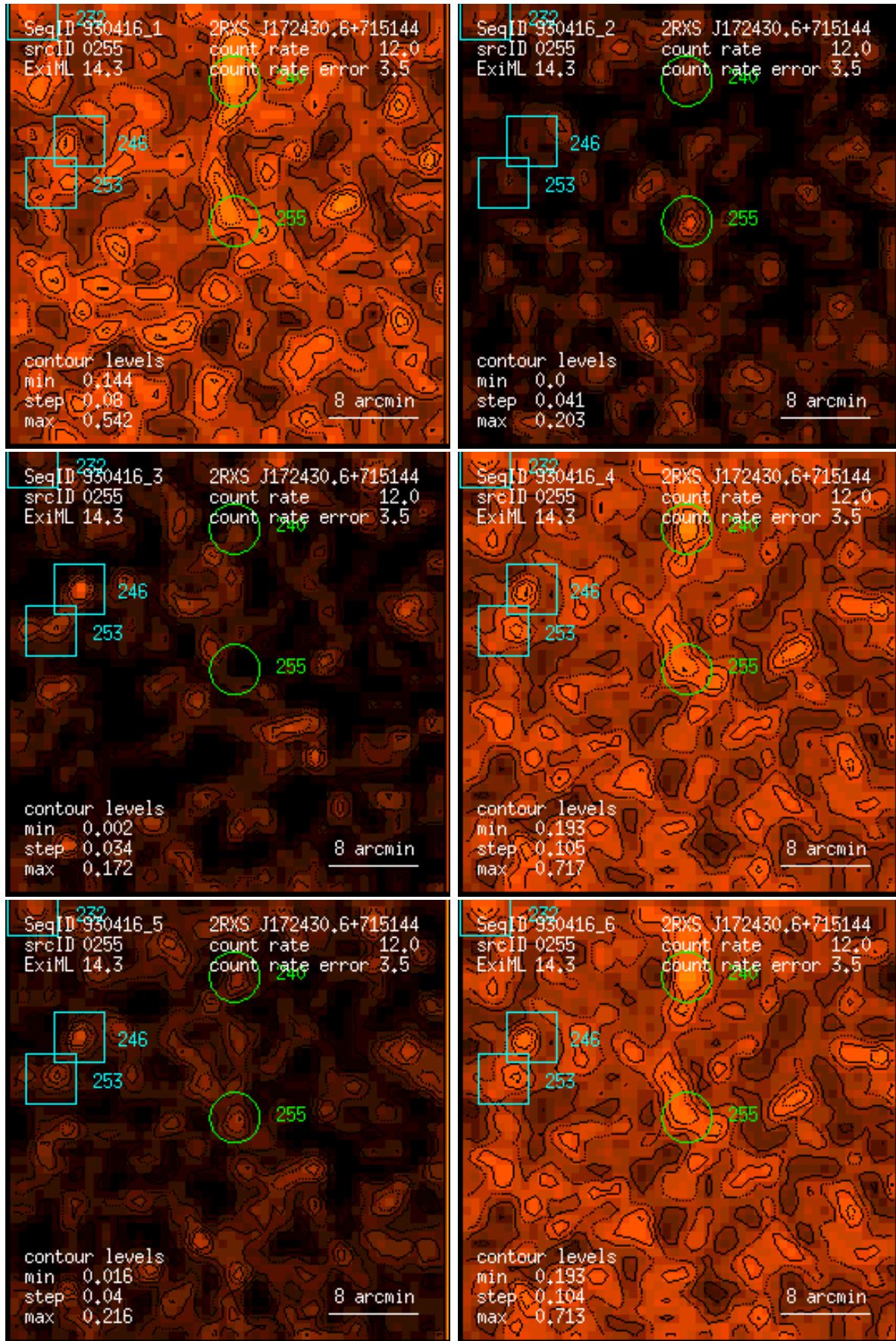
Figure 255: RASS 930416: detection 0255: band rate images, Gaussian filter: (1) PSPC channels 11 – 41, (2) 52 – 90, (3) 91 – 201, (4) 11 – 235, (5) 52 – 201, (6) 11 – 201. Broad band rates in counts/ks. Band rate contour levels in counts/ks/arcmin 2 .
