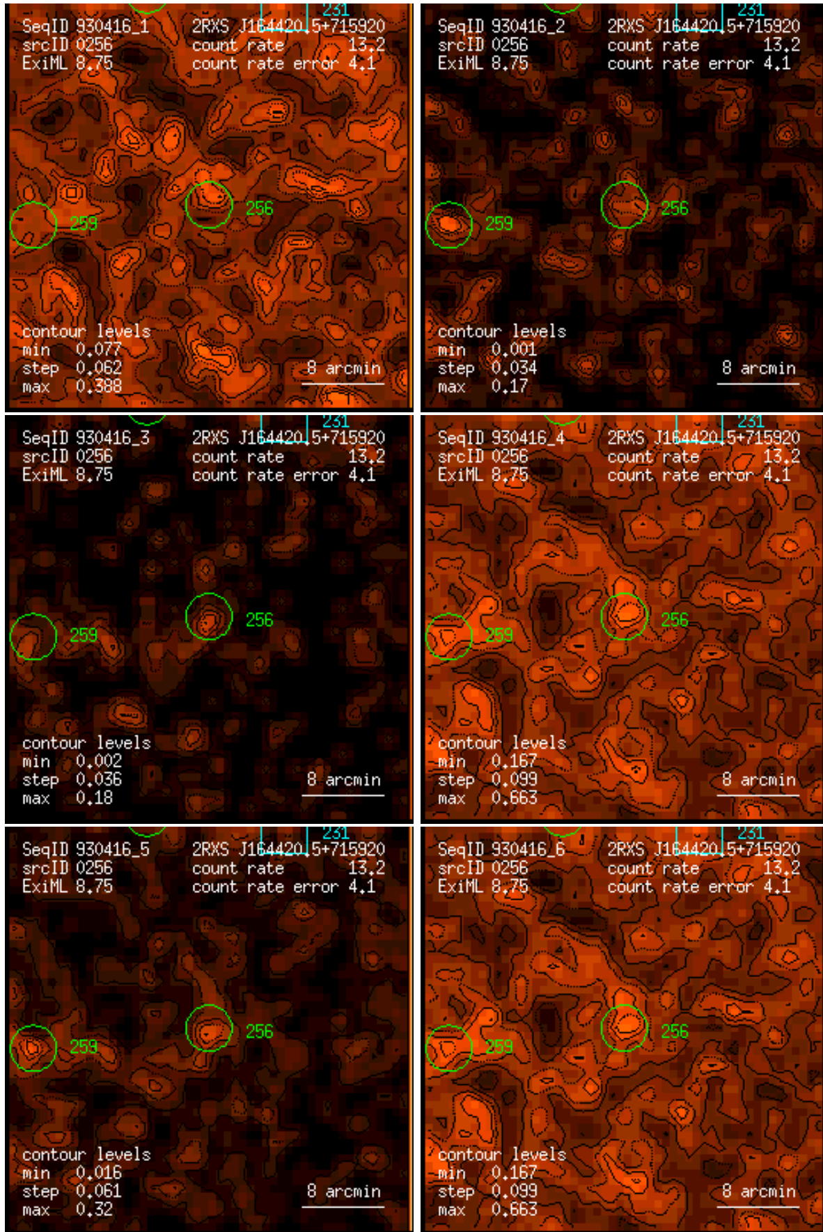
Figure 256: RASS 930416: detection 0256: band rate images, Gaussian filter: (1) PSPC channels 11 – 41, (2) 52 – 90, (3) 91 – 201, (4) 11 – 235, (5) 52 – 201, (6) 11 – 201. Broad band rates in counts/ks. Band rate contour levels in counts/ks/arcmin 2 .
