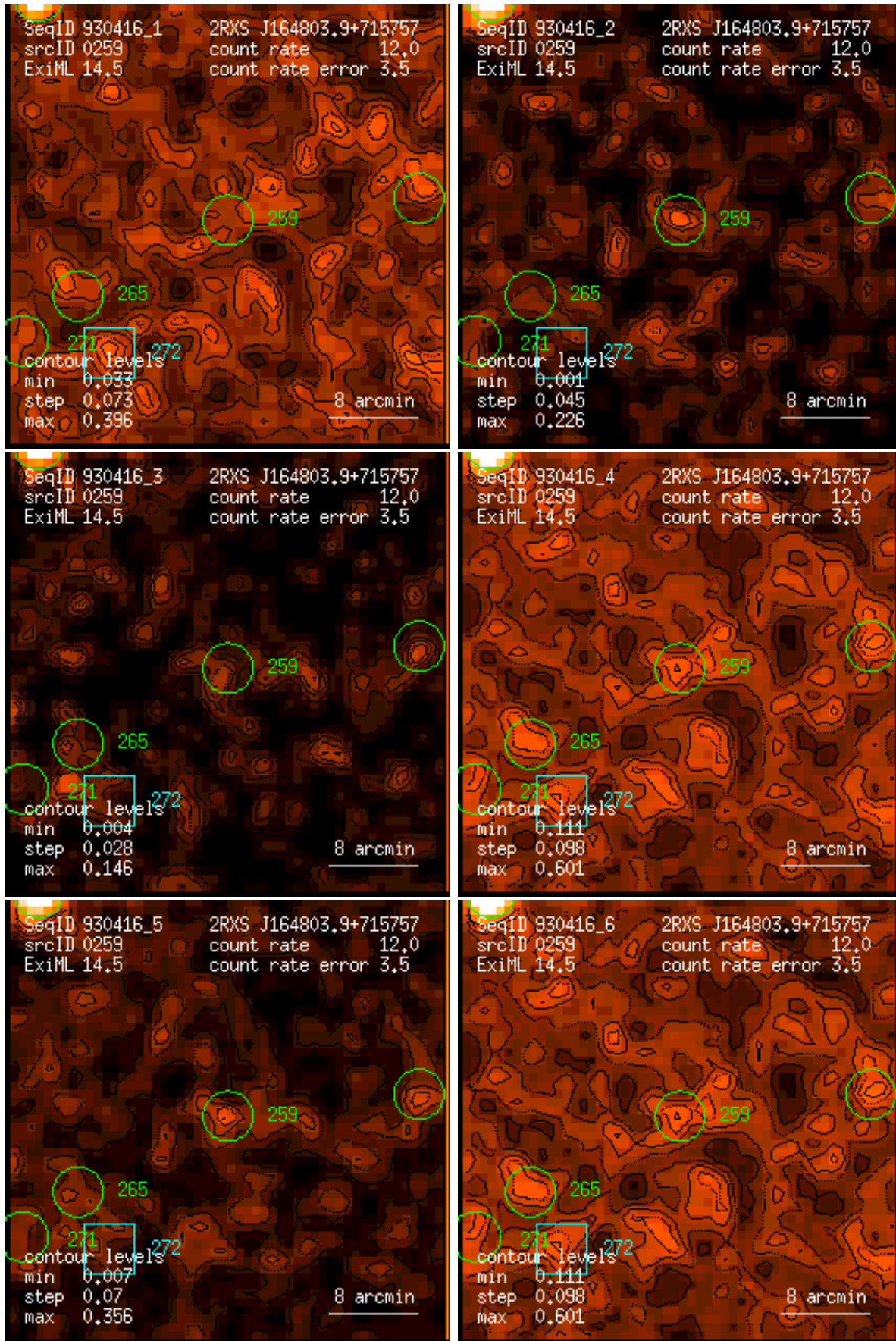
Figure 259: RASS 930416: detection 0259: band rate images, Gaussian filter: (1) PSPC channels 11 – 41, (2) 52 – 90, (3) 91 – 201, (4) 11 – 235, (5) 52 – 201, (6) 11 – 201. Broad band rates in counts/ks. Band rate contour levels in counts/ks/arcmin 2 .
