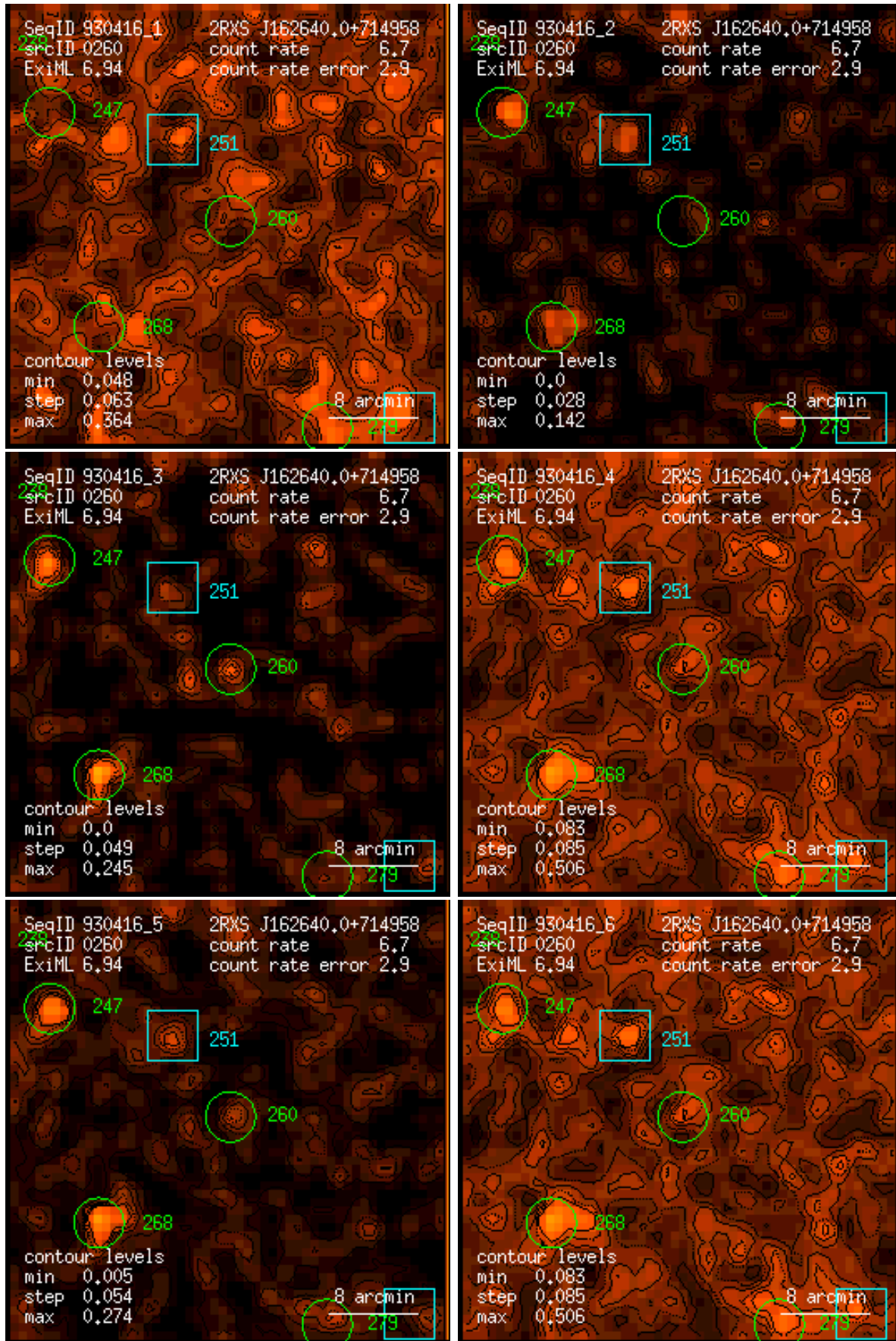
Figure 260: RASS 930416: detection 0260: band rate images, Gaussian filter: (1) PSPC channels 11 – 41, (2) 52 – 90, (3) 91 – 201, (4) 11 – 235, (5) 52 – 201, (6) 11 – 201. Broad band rates in counts/ks. Band rate contour levels in counts/ks/arcmin 2 .
