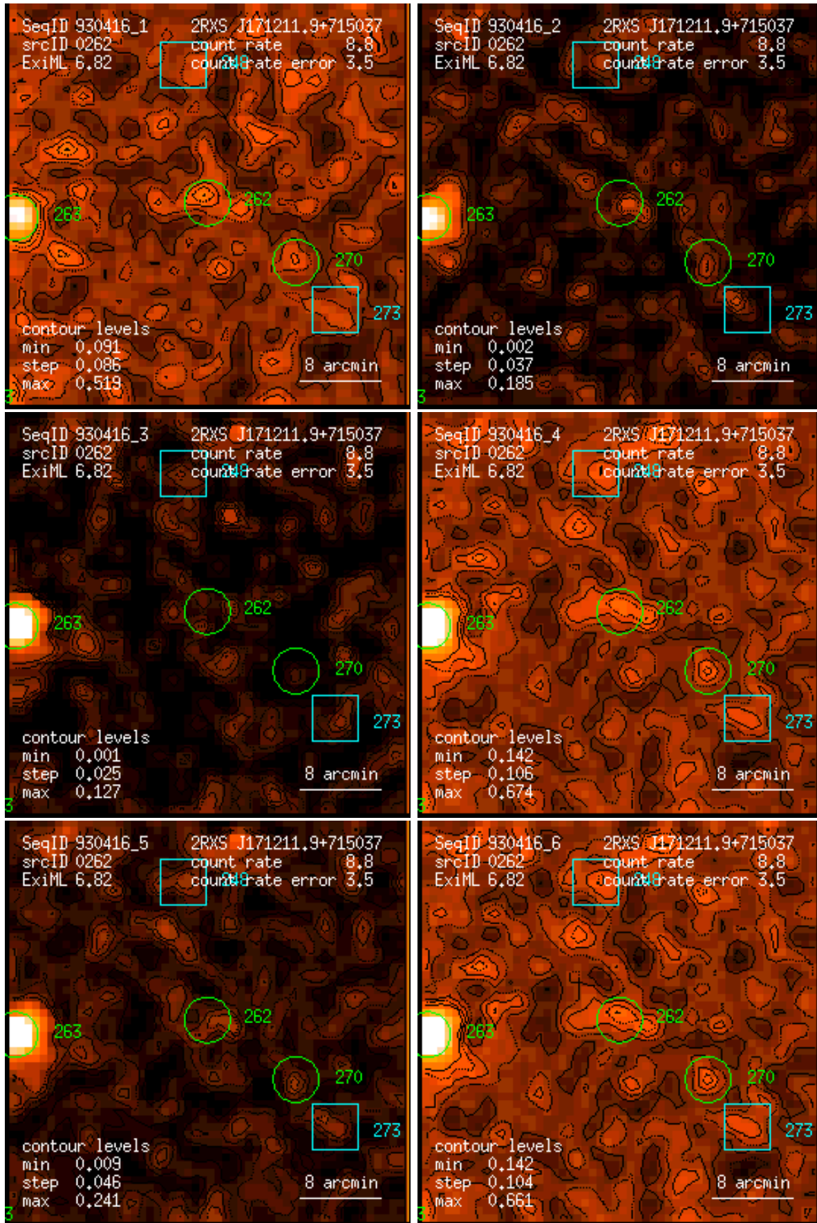
Figure 262: RASS 930416: detection 0262: band rate images, Gaussian filter: (1) PSPC channels 11 – 41, (2) 52 – 90, (3) 91 – 201, (4) 11 – 235, (5) 52 – 201, (6) 11 – 201. Broad band rates in counts/ks. Band rate contour levels in counts/ks/arcmin 2 .
