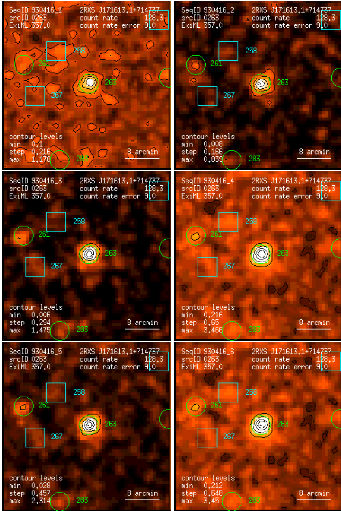
Figure 263: RASS 930416: detection 0263: band rate images, Gaussian filter: (1) PSPC channels 11 – 41, (2) 52 – 90, (3) 91 – 201, (4) 11 – 235, (5) 52 – 201, (6) 11 – 201. Broad band rates in counts/ks. Band rate contour levels in counts/ks/arcmin 2 .
