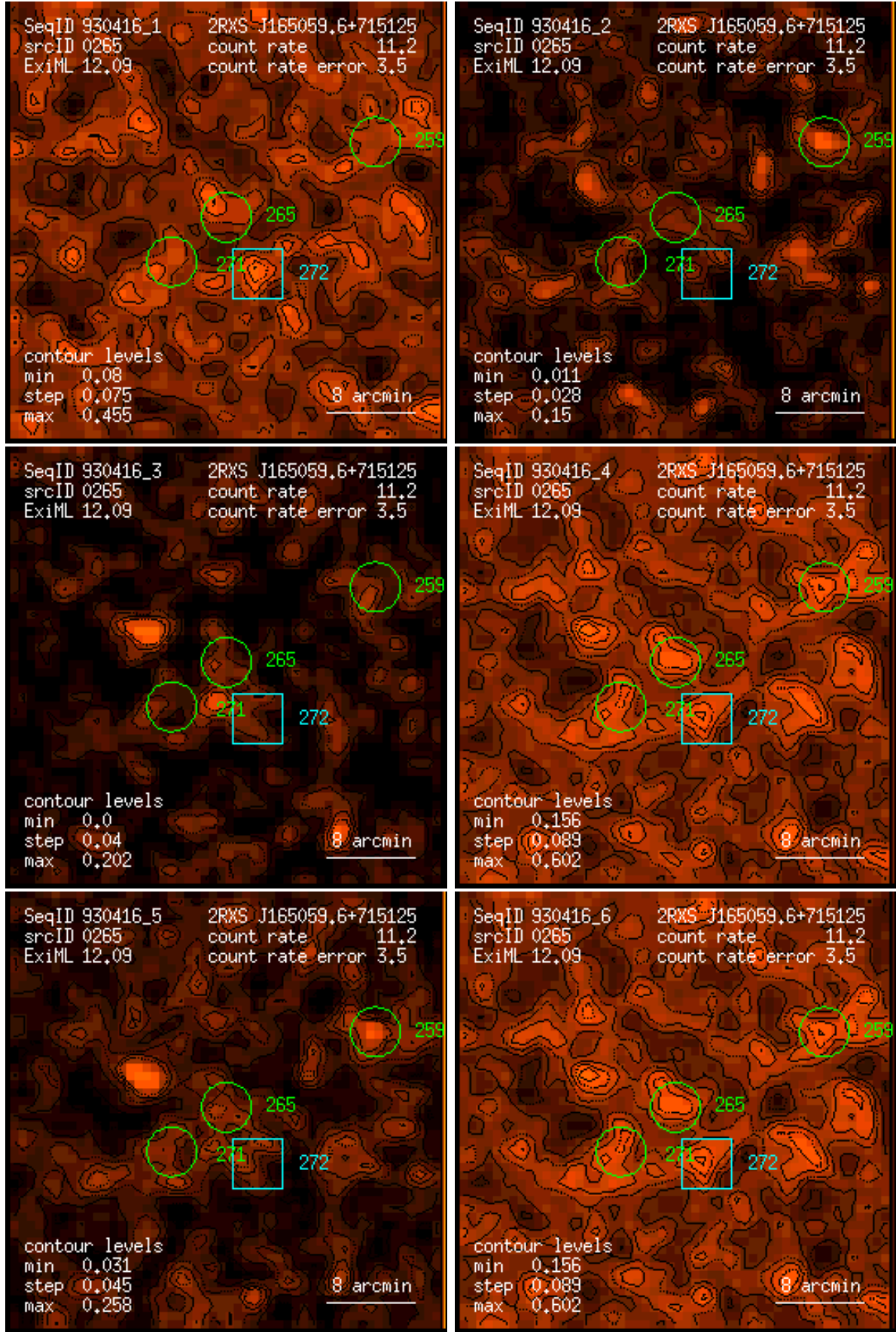
Figure 265: RASS 930416: detection 0265: band rate images, Gaussian filter: (1) PSPC channels 11 – 41, (2) 52 – 90, (3) 91 – 201, (4) 11 – 235, (5) 52 – 201, (6) 11 – 201. Broad band rates in counts/ks. Band rate contour levels in counts/ks/arcmin 2 .
