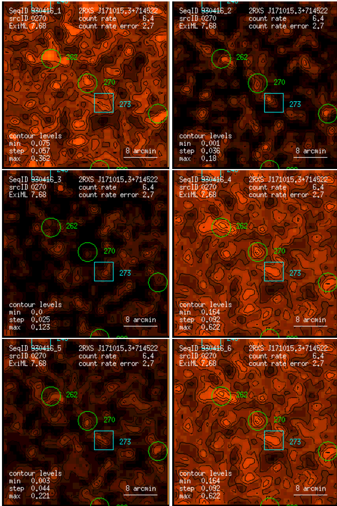
Figure 270: RASS 930416: detection 0270: band rate images, Gaussian filter: (1) PSPC channels 11 – 41, (2) 52 – 90, (3) 91 – 201, (4) 11 – 235, (5) 52 – 201, (6) 11 – 201. Broad band rates in counts/ks. Band rate contour levels in counts/ks/arcmin 2 .
