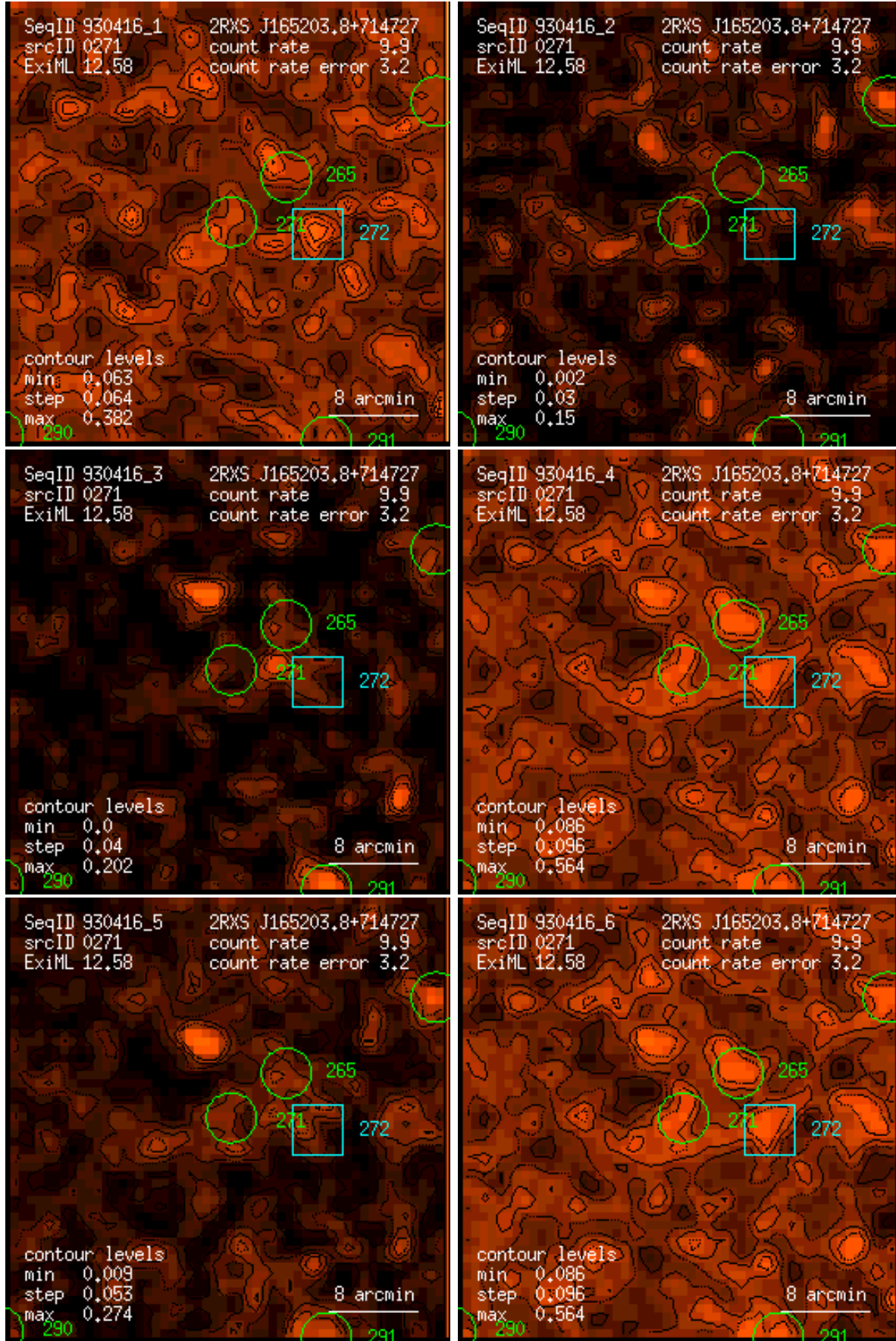
Figure 271: RASS 930416: detection 0271: band rate images, Gaussian filter: (1) PSPC channels 11 – 41, (2) 52 – 90, (3) 91 – 201, (4) 11 – 235, (5) 52 – 201, (6) 11 – 201. Broad band rates in counts/ks. Band rate contour levels in counts/ks/arcmin 2 .
