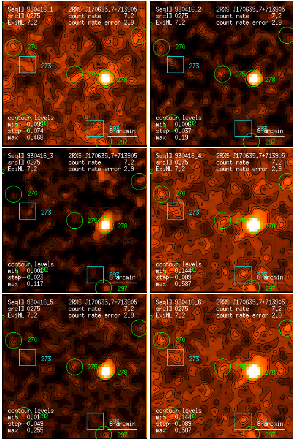
Figure 275: RASS 930416: detection 0275: band rate images, Gaussian filter: (1) PSPC channels 11 – 41, (2) 52 – 90, (3) 91 – 201, (4) 11 – 235, (5) 52 – 201, (6) 11 – 201. Broad band rates in counts/ks. Band rate contour levels in counts/ks/arcmin 2 .
