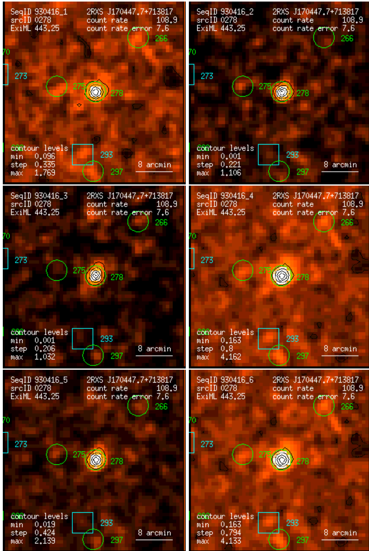
Figure 278: RASS 930416: detection 0278: band rate images, Gaussian filter: (1) PSPC channels 11 – 41, (2) 52 – 90, (3) 91 – 201, (4) 11 – 235, (5) 52 – 201, (6) 11 – 201. Broad band rates in counts/ks. Band rate contour levels in counts/ks/arcmin 2 .
