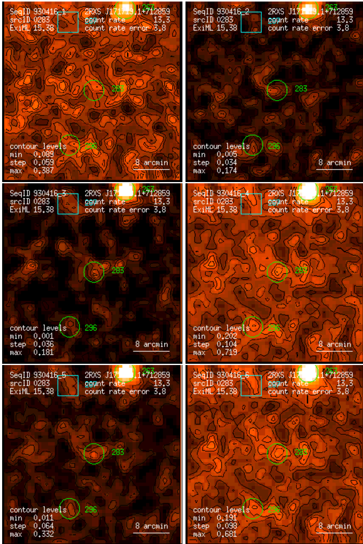
Figure 283: RASS 930416: detection 0283: band rate images, Gaussian filter: (1) PSPC channels 11 – 41, (2) 52 – 90, (3) 91 – 201, (4) 11 – 235, (5) 52 – 201, (6) 11 – 201. Broad band rates in counts/ks. Band rate contour levels in counts/ks/arcmin 2 .
