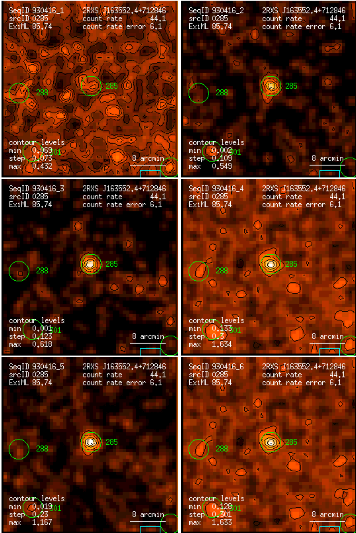
Figure 285: RASS 930416: detection 0285: band rate images, Gaussian filter: (1) PSPC channels 11 – 41, (2) 52 – 90, (3) 91 – 201, (4) 11 – 235, (5) 52 – 201, (6) 11 – 201. Broad band rates in counts/ks. Band rate contour levels in counts/ks/arcmin 2 .
