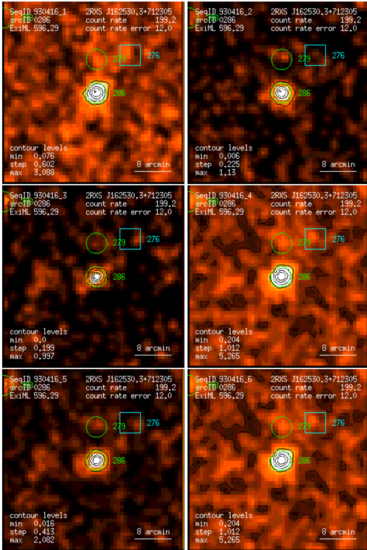
Figure 286: RASS 930416: detection 0286: band rate images, Gaussian filter: (1) PSPC channels 11 – 41, (2) 52 – 90, (3) 91 – 201, (4) 11 – 235, (5) 52 – 201, (6) 11 – 201. Broad band rates in counts/ks. Band rate contour levels in counts/ks/arcmin 2 .
