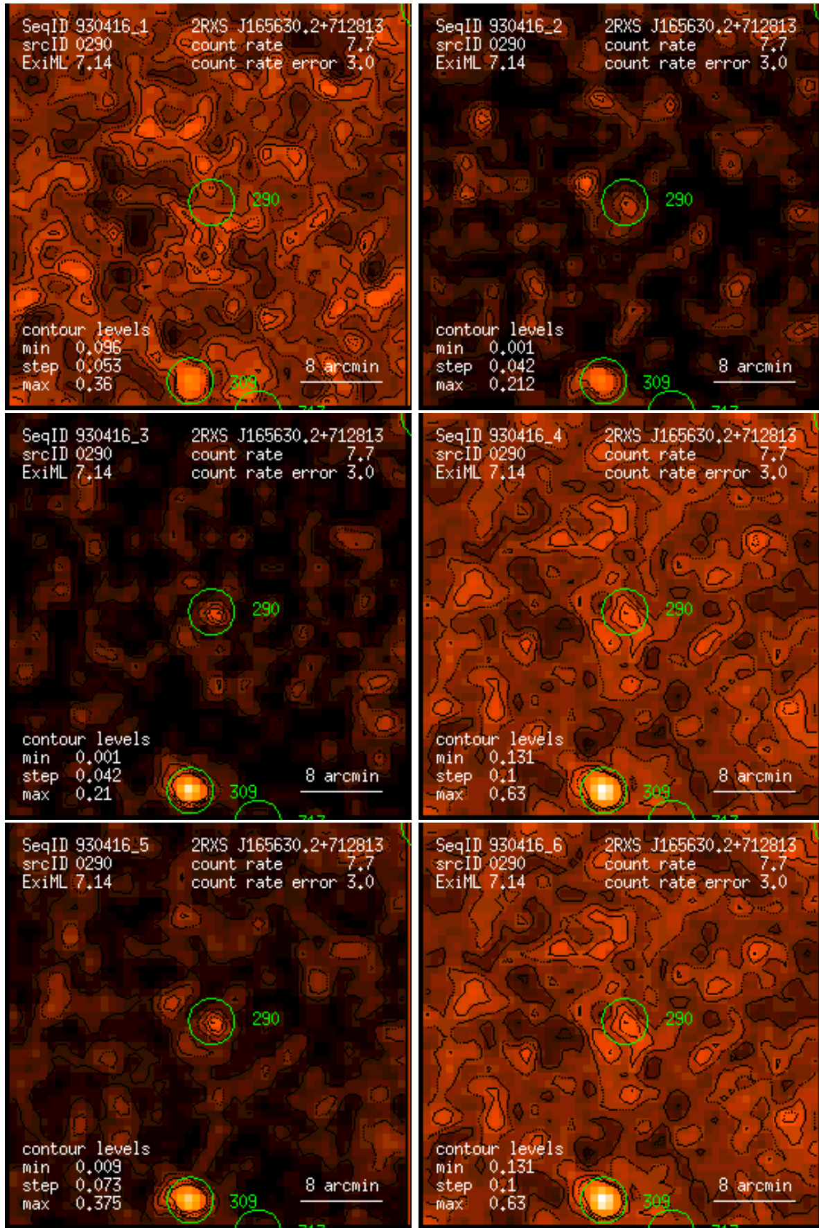
Figure 290: RASS 930416: detection 0290: band rate images, Gaussian filter: (1) PSPC channels 11 – 41, (2) 52 – 90, (3) 91 – 201, (4) 11 – 235, (5) 52 – 201, (6) 11 – 201. Broad band rates in counts/ks. Band rate contour levels in counts/ks/arcmin 2 .
