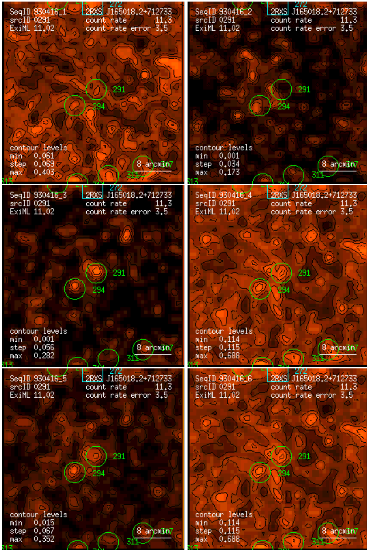
Figure 291: RASS 930416: detection 0291: band rate images, Gaussian filter: (1) PSPC channels 11 – 41, (2) 52 – 90, (3) 91 – 201, (4) 11 – 235, (5) 52 – 201, (6) 11 – 201. Broad band rates in counts/ks. Band rate contour levels in counts/ks/arcmin 2 .
