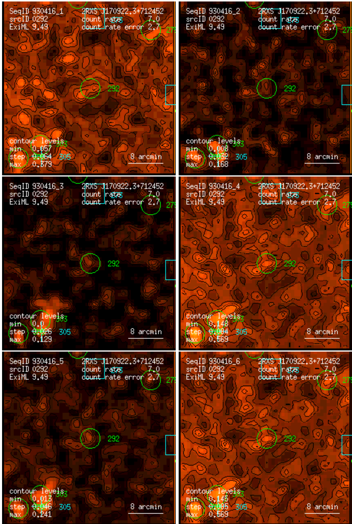
Figure 292: RASS 930416: detection 0292: band rate images, Gaussian filter: (1) PSPC channels 11 – 41, (2) 52 – 90, (3) 91 – 201, (4) 11 – 235, (5) 52 – 201, (6) 11 – 201. Broad band rates in counts/ks. Band rate contour levels in counts/ks/arcmin 2 .
