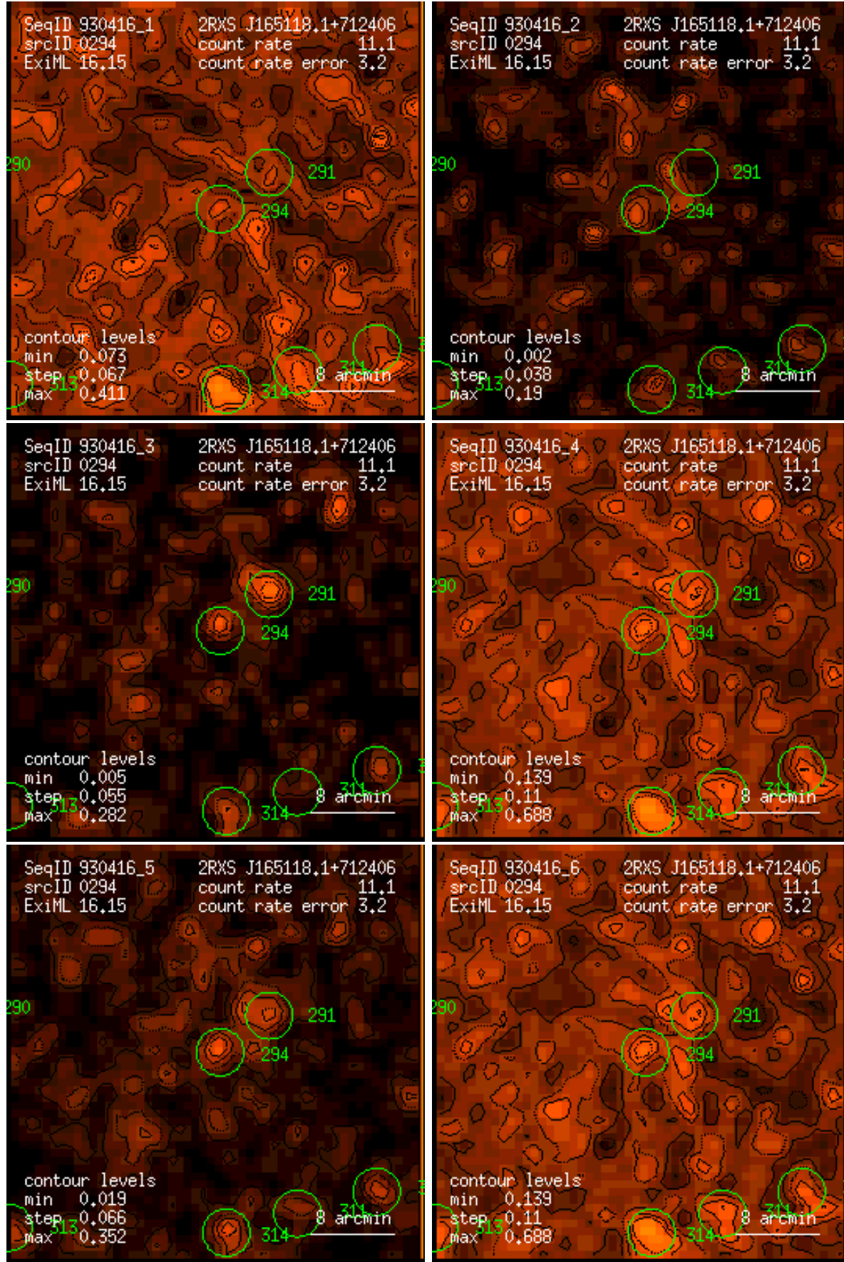
Figure 294: RASS 930416: detection 0294: band rate images, Gaussian filter: (1) PSPC channels 11 – 41, (2) 52 – 90, (3) 91 – 201, (4) 11 – 235, (5) 52 – 201, (6) 11 – 201. Broad band rates in counts/ks. Band rate contour levels in counts/ks/arcmin 2 .
