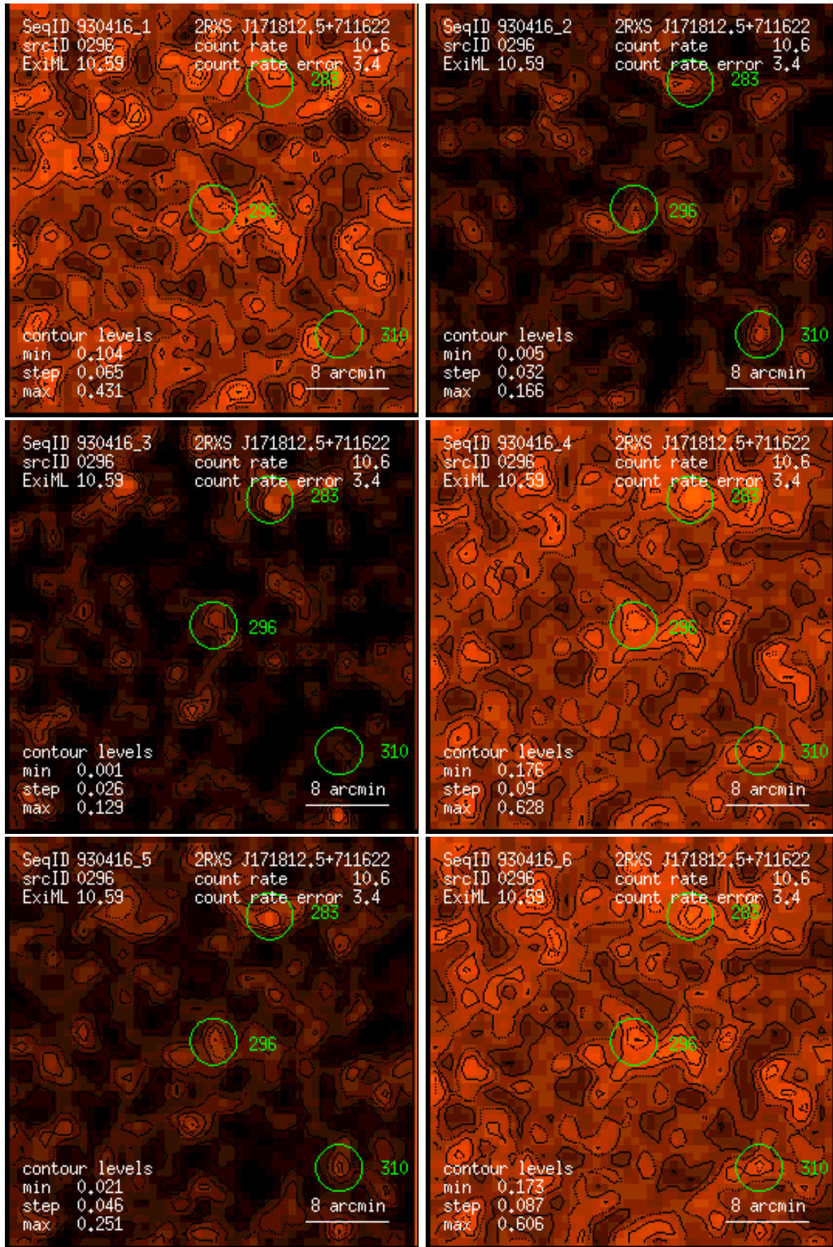
Figure 296: RASS 930416: detection 0296: band rate images, Gaussian filter: (1) PSPC channels 11 – 41, (2) 52 – 90, (3) 91 – 201, (4) 11 – 235, (5) 52 – 201, (6) 11 – 201. Broad band rates in counts/ks. Band rate contour levels in counts/ks/arcmin 2 .
