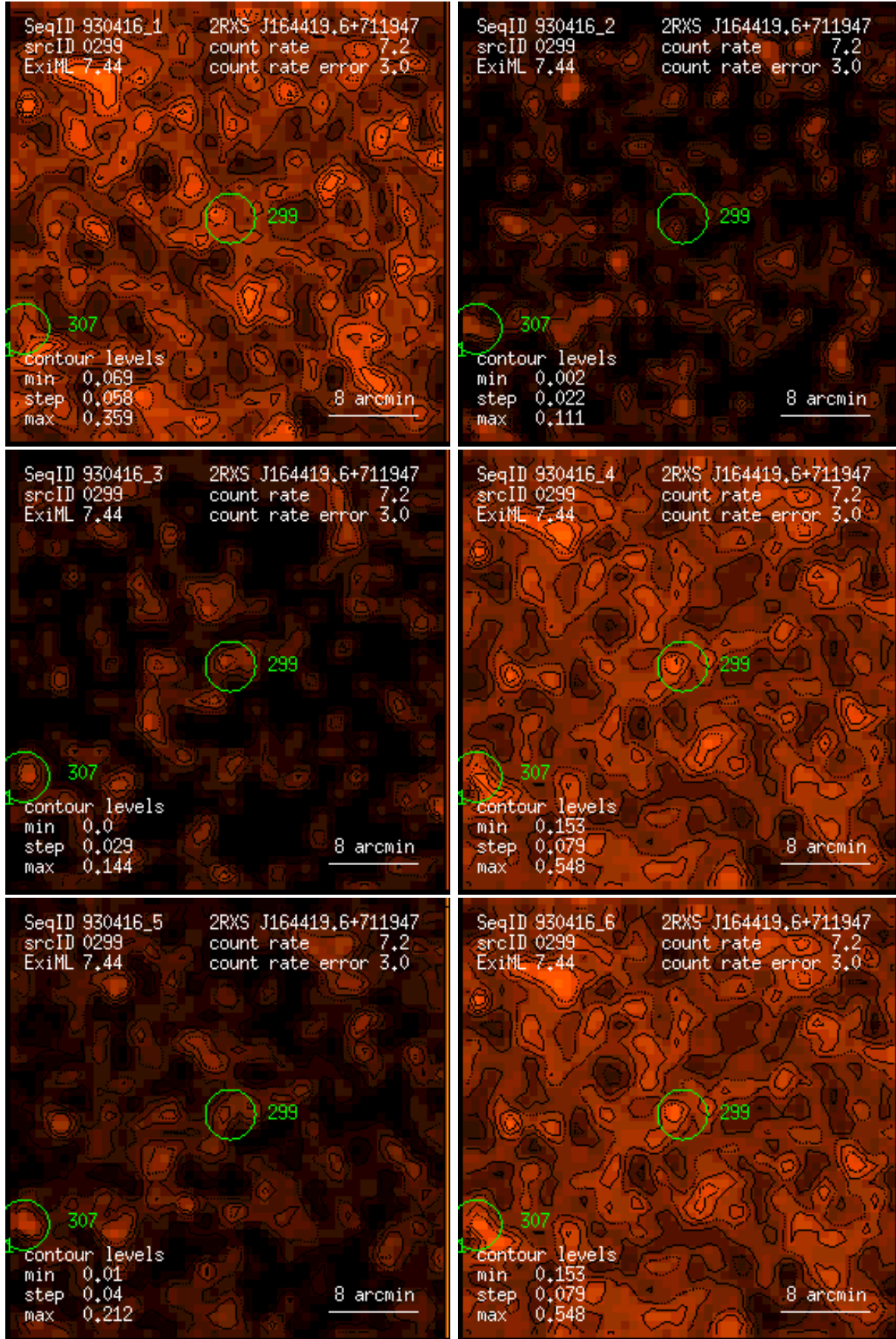
Figure 299: RASS 930416: detection 0299: band rate images, Gaussian filter: (1) PSPC channels 11 – 41, (2) 52 – 90, (3) 91 – 201, (4) 11 – 235, (5) 52 – 201, (6) 11 – 201. Broad band rates in counts/ks. Band rate contour levels in counts/ks/arcmin 2 .
