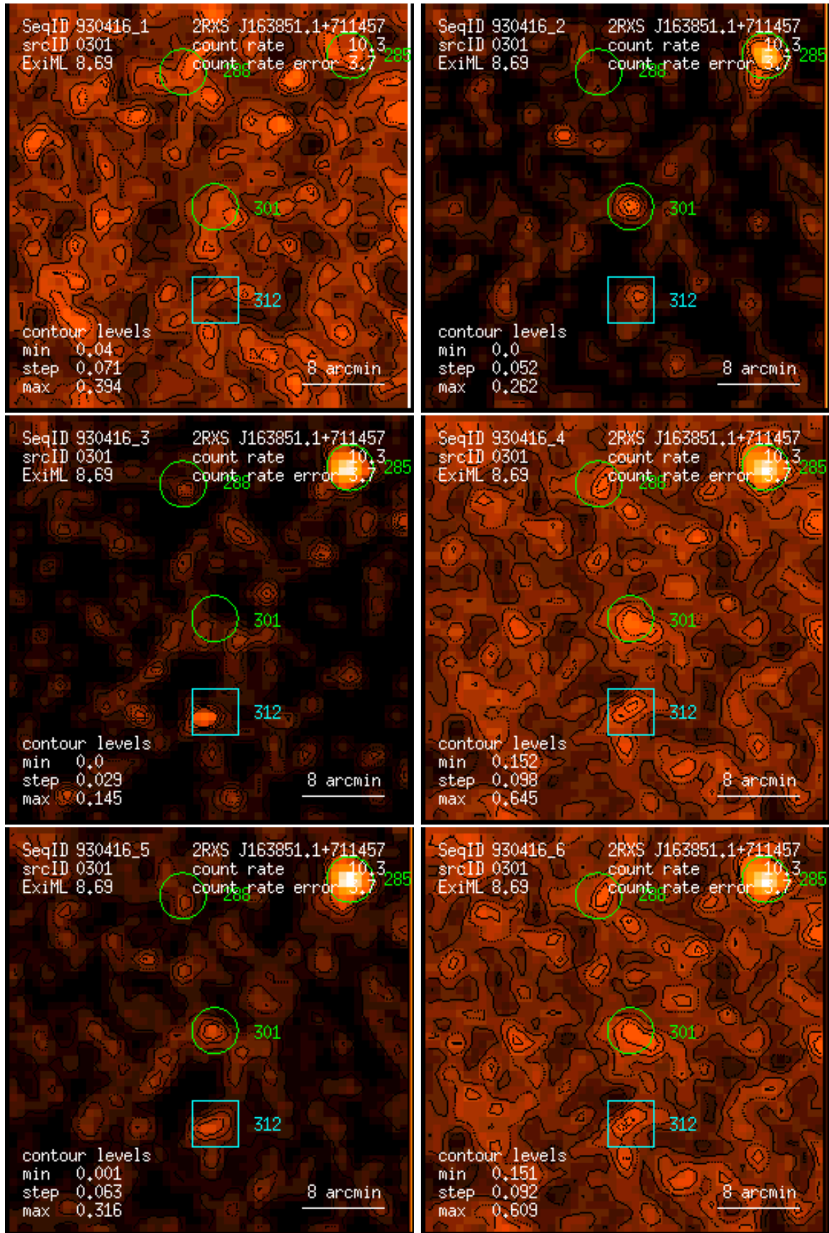
Figure 301: RASS 930416: detection 0301: band rate images, Gaussian filter: (1) PSPC channels 11 – 41, (2) 52 – 90, (3) 91 – 201, (4) 11 – 235, (5) 52 – 201, (6) 11 – 201. Broad band rates in counts/ks. Band rate contour levels in counts/ks/arcmin 2 .
