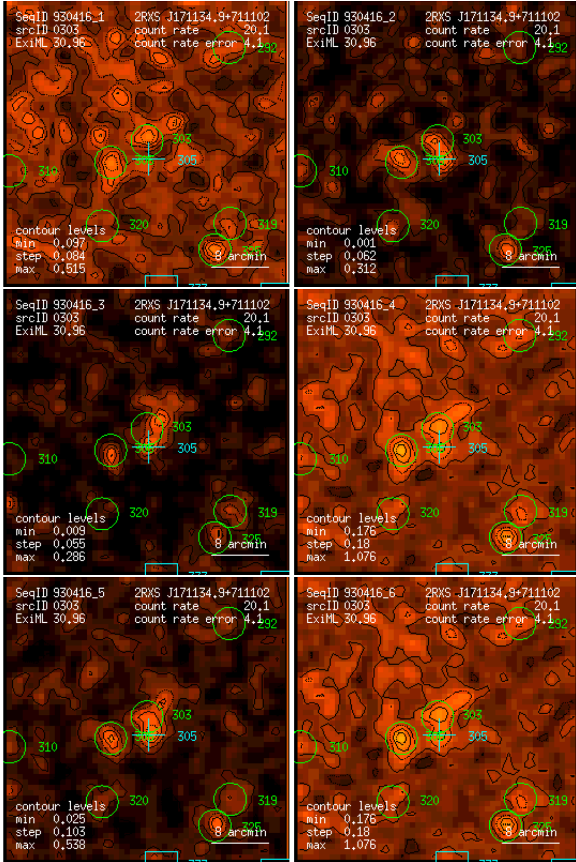
Figure 303: RASS 930416: detection 0303: band rate images, Gaussian filter: (1) PSPC channels 11 – 41, (2) 52 – 90, (3) 91 – 201, (4) 11 – 235, (5) 52 – 201, (6) 11 – 201. Broad band rates in counts/ks. Band rate contour levels in counts/ks/arcmin 2 .
