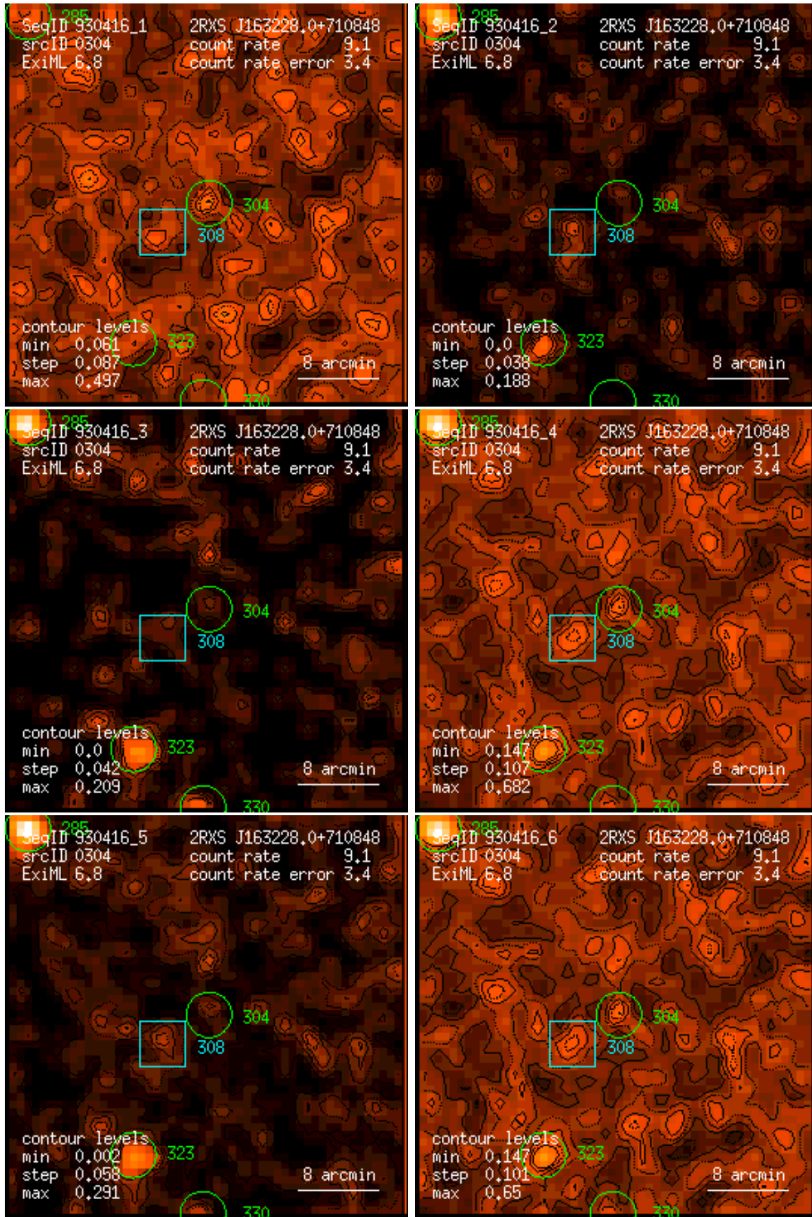
Figure 304: RASS 930416: detection 0304: band rate images, Gaussian filter: (1) PSPC channels 11 – 41, (2) 52 – 90, (3) 91 – 201, (4) 11 – 235, (5) 52 – 201, (6) 11 – 201. Broad band rates in counts/ks. Band rate contour levels in counts/ks/arcmin 2 .
