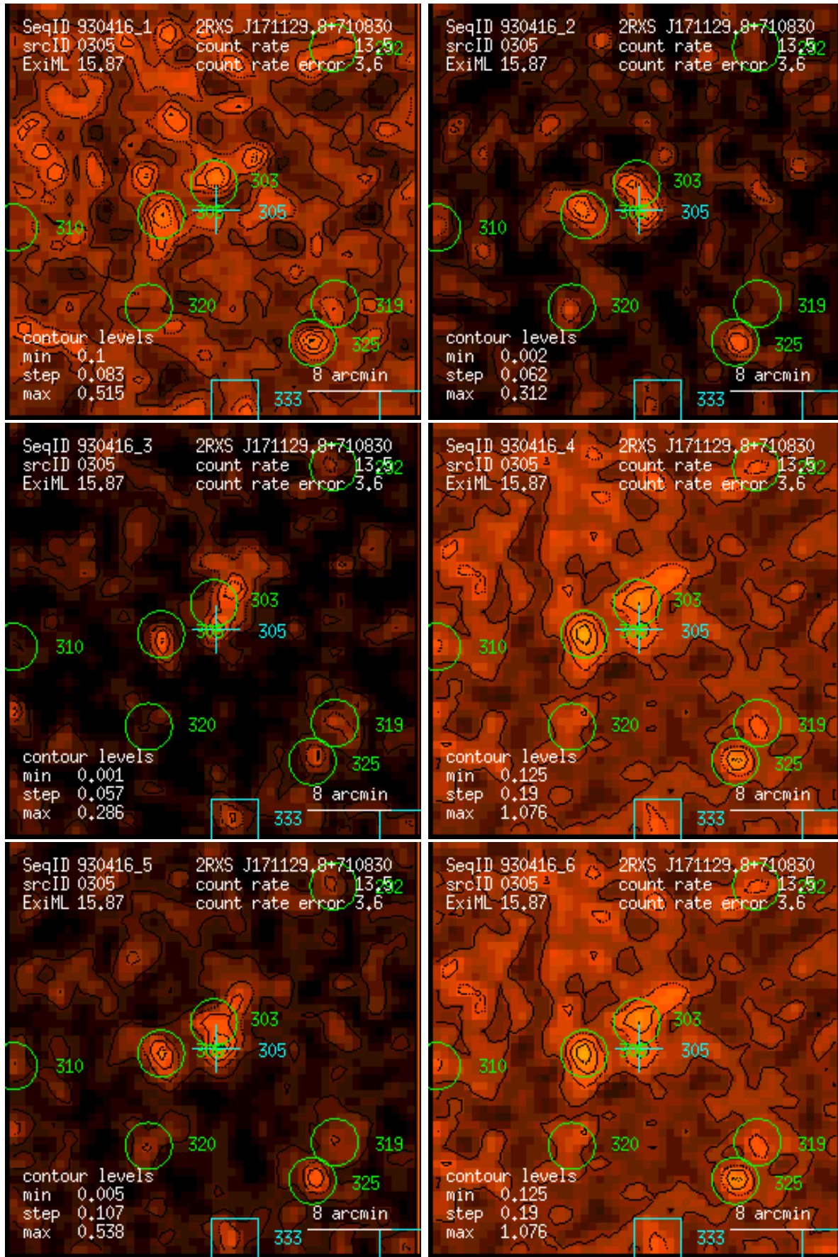
Figure 305: RASS 930416: detection 0305: band rate images, Gaussian filter: (1) PSPC channels 11 – 41, (2) 52 – 90, (3) 91 – 201, (4) 11 – 235, (5) 52 – 201, (6) 11 – 201. Broad band rates in counts/ks. Band rate contour levels in counts/ks/arcmin 2 .
