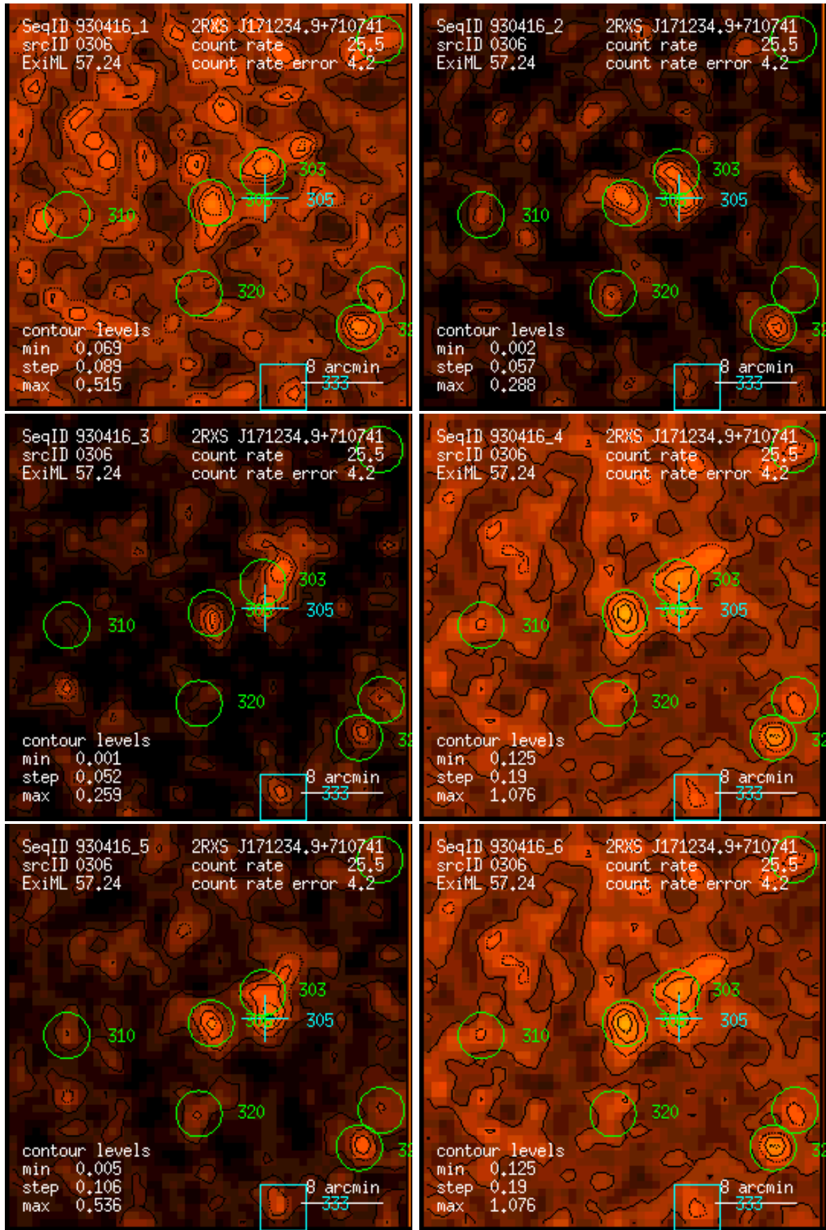
Figure 306: RASS 930416: detection 0306: band rate images, Gaussian filter: (1) PSPC channels 11 – 41, (2) 52 – 90, (3) 91 – 201, (4) 11 – 235, (5) 52 – 201, (6) 11 – 201. Broad band rates in counts/ks. Band rate contour levels in counts/ks/arcmin 2 .
