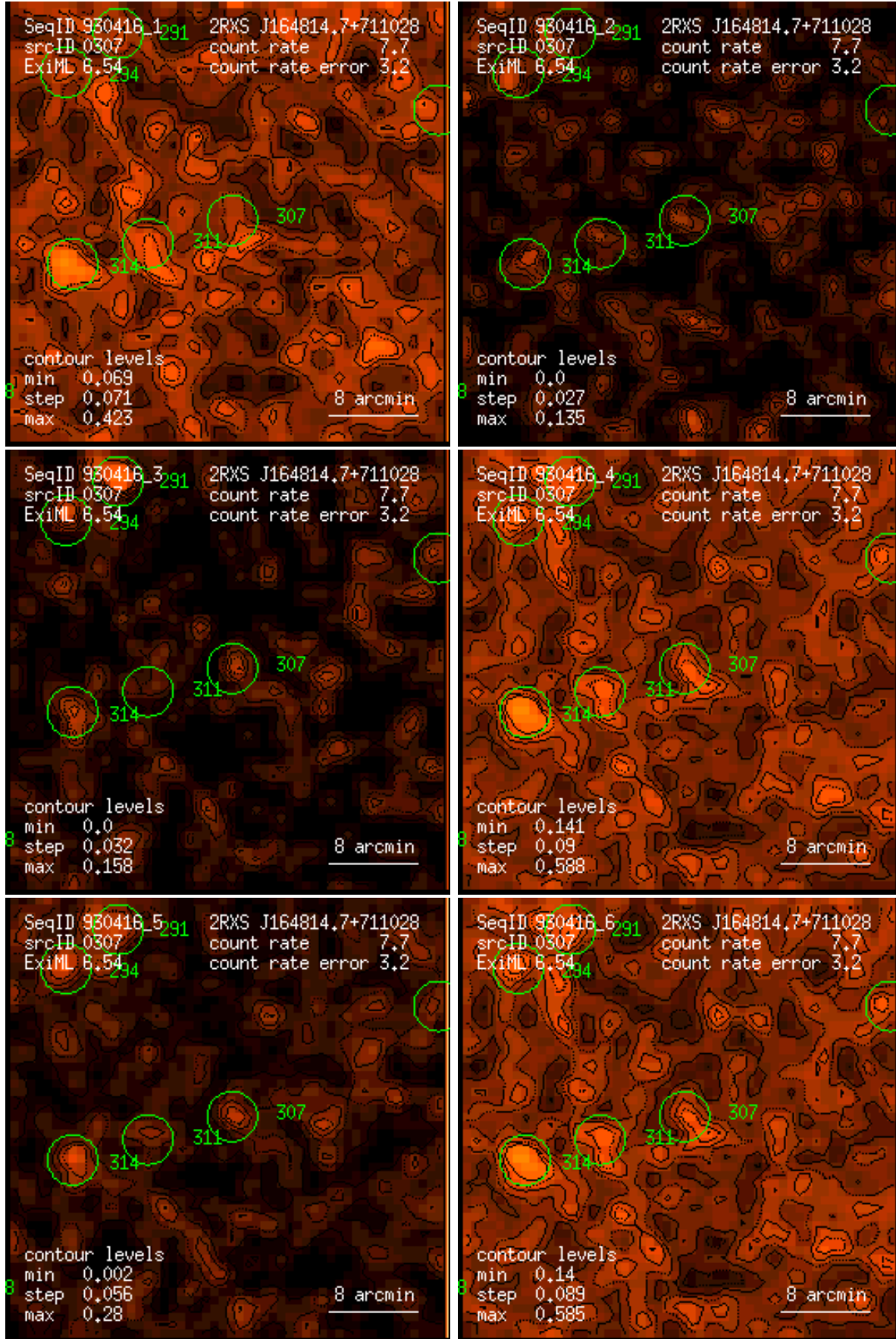
Figure 307: RASS 930416: detection 0307: band rate images, Gaussian filter: (1) PSPC channels 11 – 41, (2) 52 – 90, (3) 91 – 201, (4) 11 – 235, (5) 52 – 201, (6) 11 – 201. Broad band rates in counts/ks. Band rate contour levels in counts/ks/arcmin 2 .
