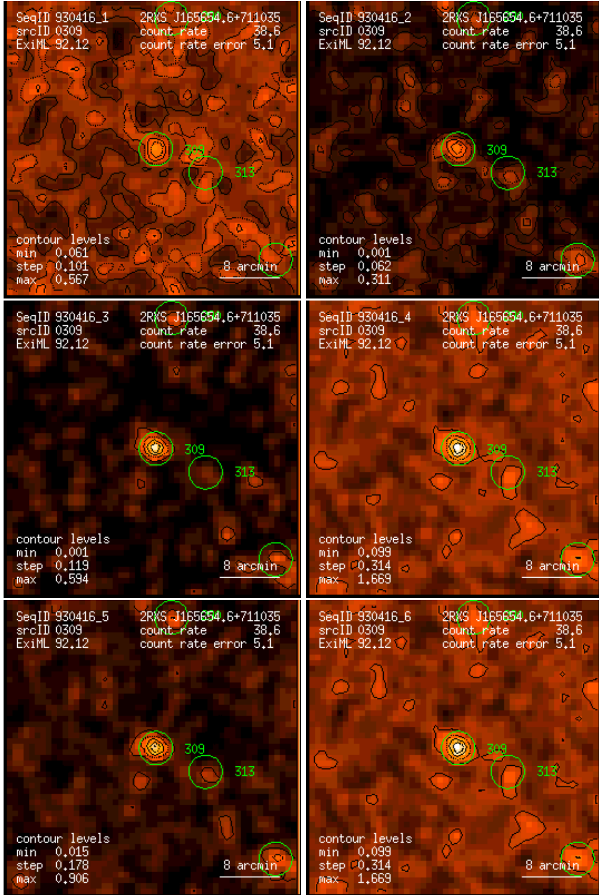
Figure 309: RASS 930416: detection 0309: band rate images, Gaussian filter: (1) PSPC channels 11 – 41, (2) 52 – 90, (3) 91 – 201, (4) 11 – 235, (5) 52 – 201, (6) 11 – 201. Broad band rates in counts/ks. Band rate contour levels in counts/ks/arcmin 2 .
