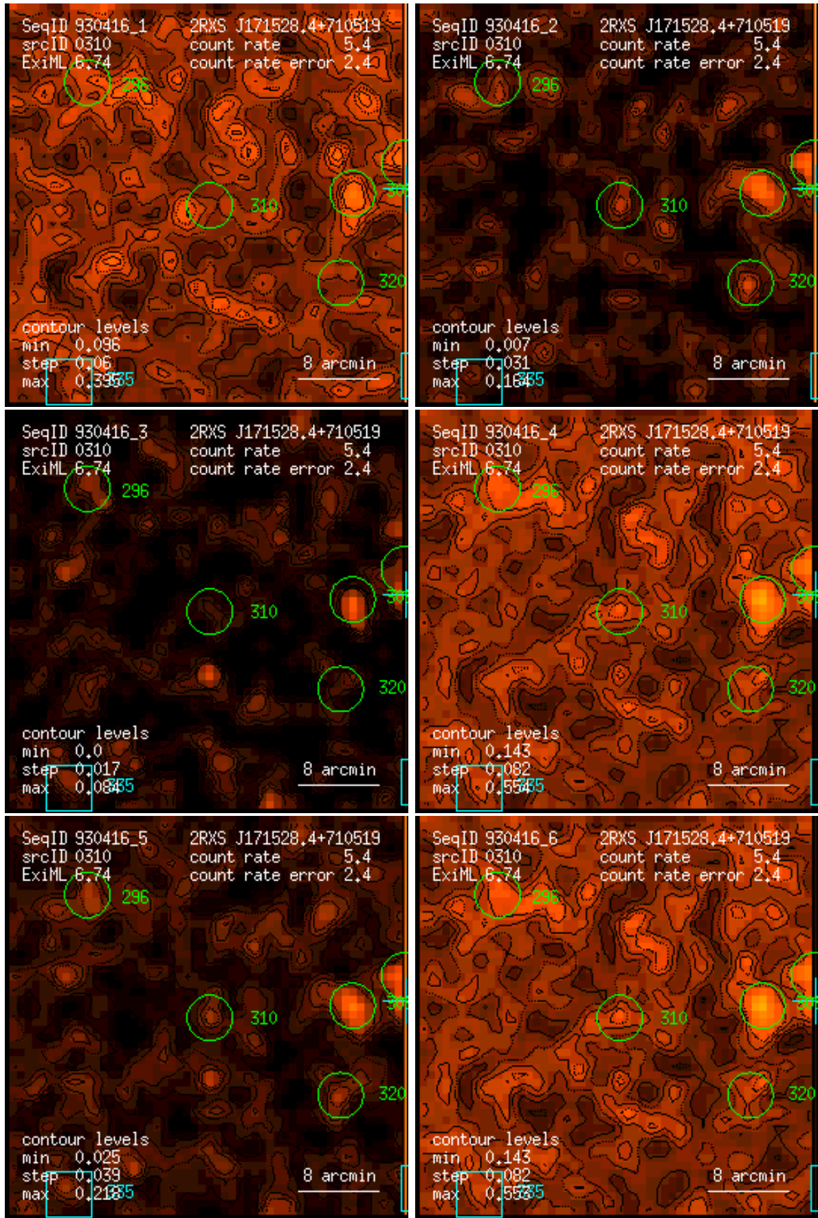
Figure 310: RASS 930416: detection 0310: band rate images, Gaussian filter: (1) PSPC channels 11 – 41, (2) 52 – 90, (3) 91 – 201, (4) 11 – 235, (5) 52 – 201, (6) 11 – 201. Broad band rates in counts/ks. Band rate contour levels in counts/ks/arcmin 2 .
