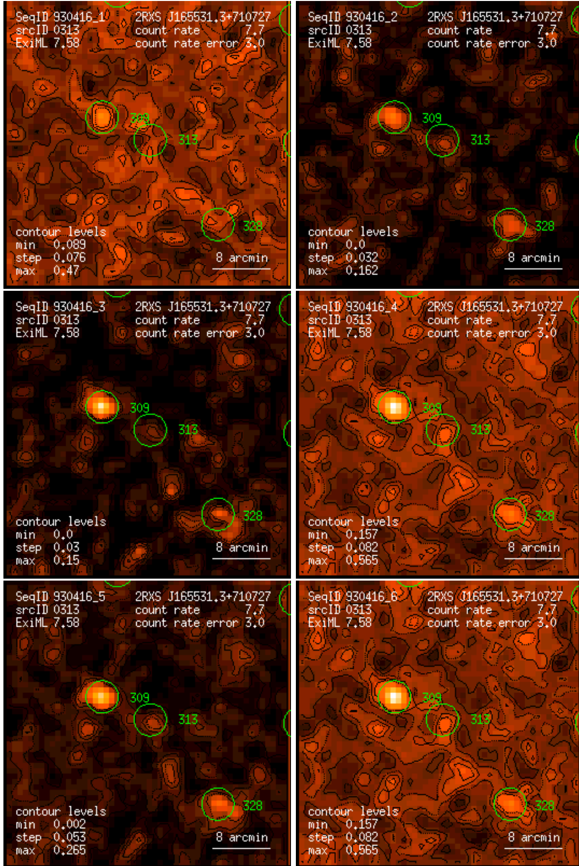
Figure 313: RASS 930416: detection 0313: band rate images, Gaussian filter: (1) PSPC channels 11 – 41, (2) 52 – 90, (3) 91 – 201, (4) 11 – 235, (5) 52 – 201, (6) 11 – 201. Broad band rates in counts/ks. Band rate contour levels in counts/ks/arcmin 2 .
