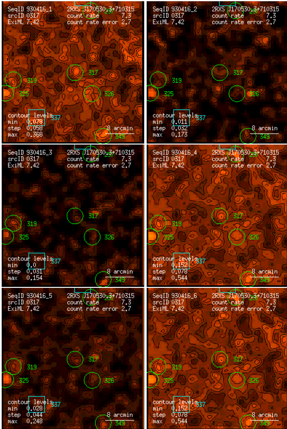
Figure 317: RASS 930416: detection 0317: band rate images, Gaussian filter: (1) PSPC channels 11 – 41, (2) 52 – 90, (3) 91 – 201, (4) 11 – 235, (5) 52 – 201, (6) 11 – 201. Broad band rates in counts/ks. Band rate contour levels in counts/ks/arcmin 2 .
