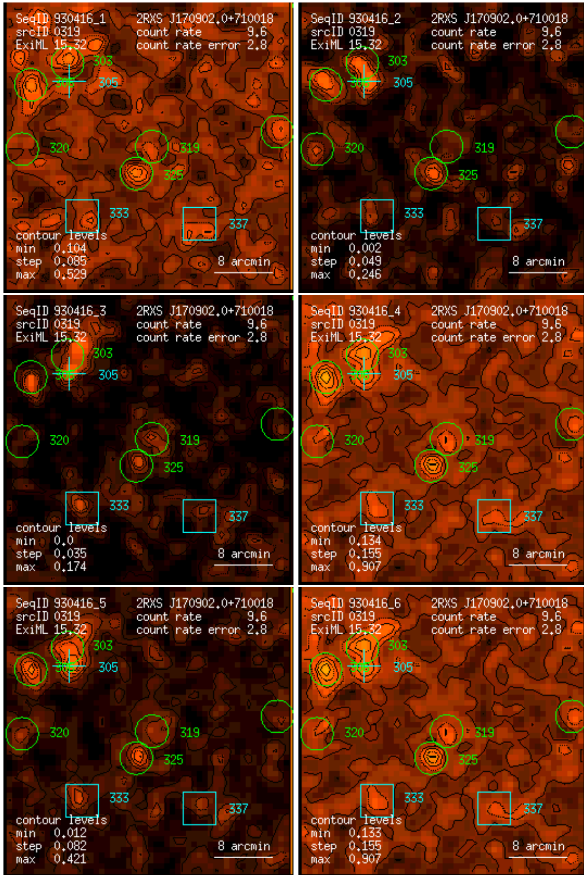
Figure 319: RASS 930416: detection 0319: band rate images, Gaussian filter: (1) PSPC channels 11 – 41, (2) 52 – 90, (3) 91 – 201, (4) 11 – 235, (5) 52 – 201, (6) 11 – 201. Broad band rates in counts/ks. Band rate contour levels in counts/ks/arcmin 2 .
