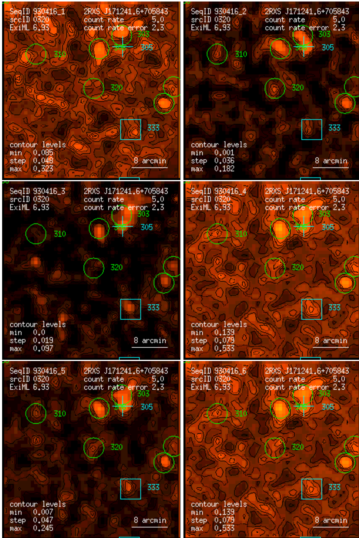
Figure 320: RASS 930416: detection 0320: band rate images, Gaussian filter: (1) PSPC channels 11 – 41, (2) 52 – 90, (3) 91 – 201, (4) 11 – 235, (5) 52 – 201, (6) 11 – 201. Broad band rates in counts/ks. Band rate contour levels in counts/ks/arcmin 2 .
