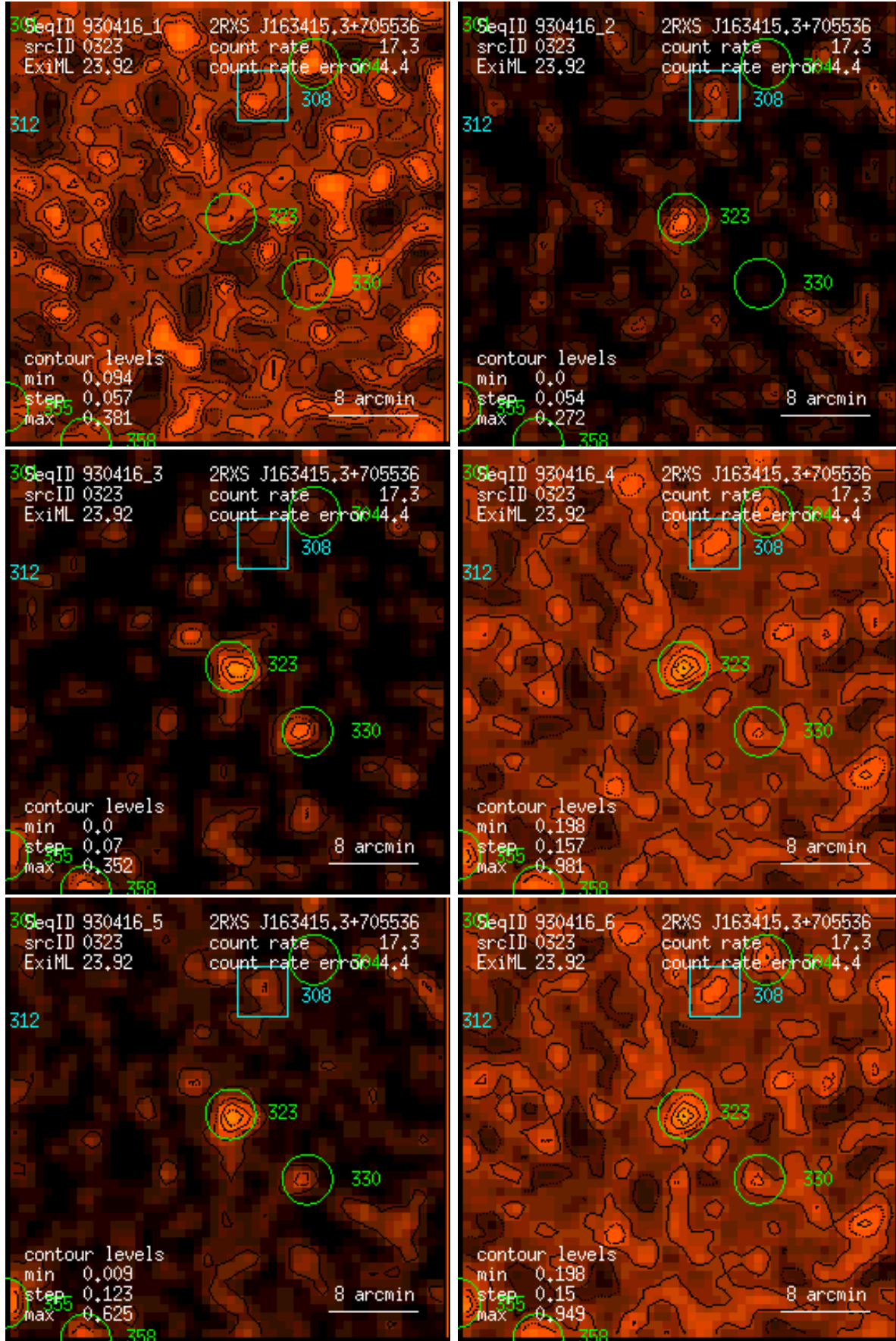
Figure 323: RASS 930416: detection 0323: band rate images, Gaussian filter: (1) PSPC channels 11 – 41, (2) 52 – 90, (3) 91 – 201, (4) 11 – 235, (5) 52 – 201, (6) 11 – 201. Broad band rates in counts/ks. Band rate contour levels in counts/ks/arcmin 2 .
