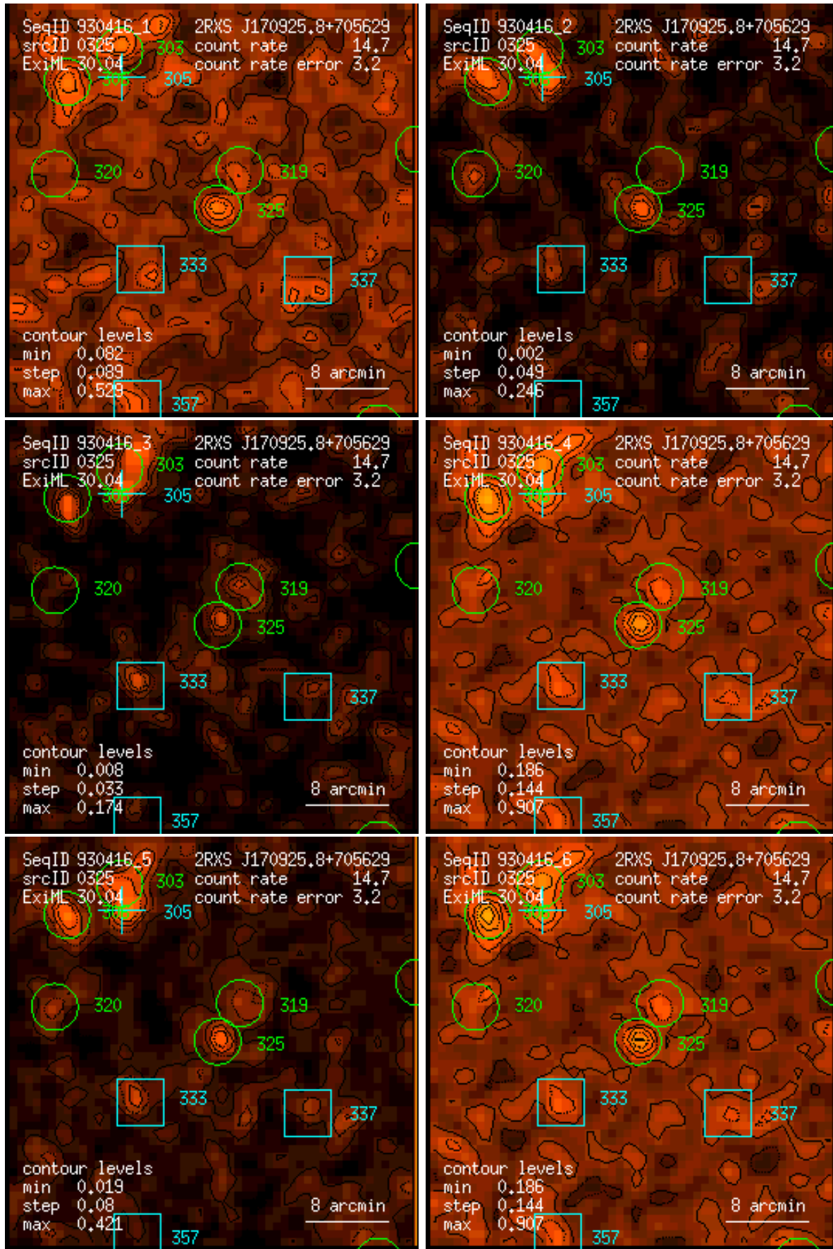
Figure 325: RASS 930416: detection 0325: band rate images, Gaussian filter: (1) PSPC channels 11 – 41, (2) 52 – 90, (3) 91 – 201, (4) 11 – 235, (5) 52 – 201, (6) 11 – 201. Broad band rates in counts/ks. Band rate contour levels in counts/ks/arcmin 2 .
