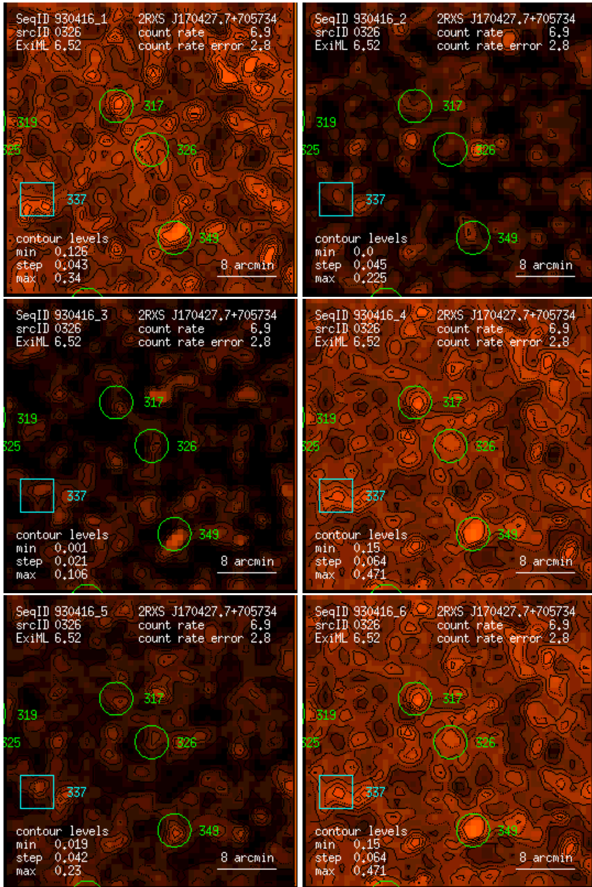
Figure 326: RASS 930416: detection 0326: band rate images, Gaussian filter: (1) PSPC channels 11 – 41, (2) 52 – 90, (3) 91 – 201, (4) 11 – 235, (5) 52 – 201, (6) 11 – 201. Broad band rates in counts/ks. Band rate contour levels in counts/ks/arcmin 2 .
